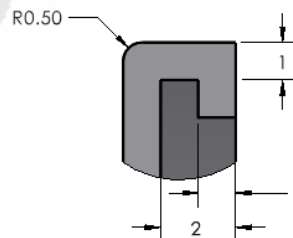
DETAIL C SCALE 8 : 1
