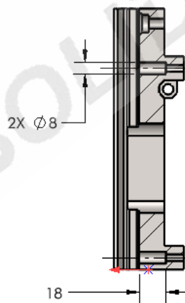
SECTION G-G
