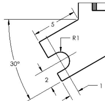
DETAIL E SCALE 6 : 1
