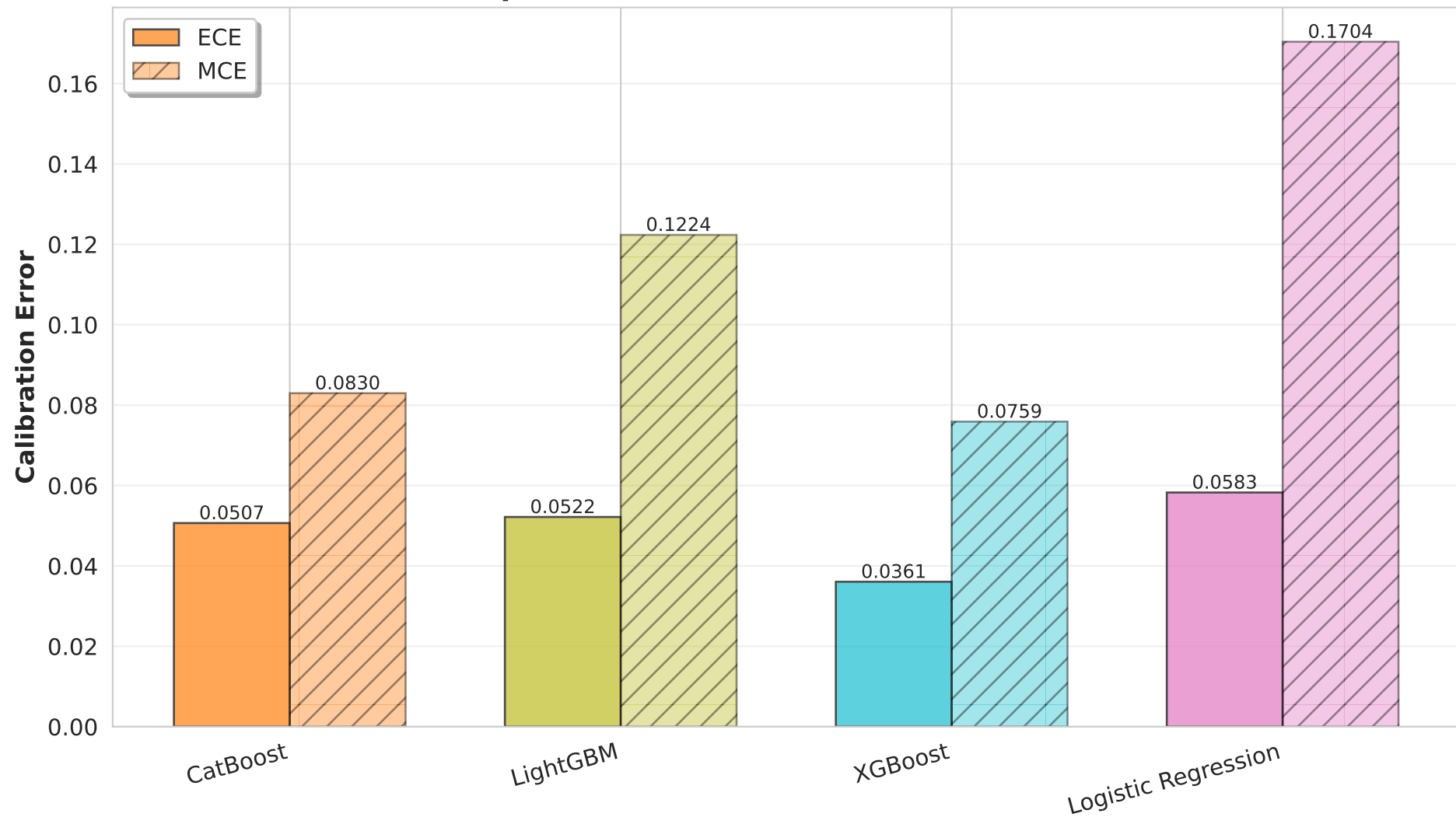
Expected vs Maximum Calibration Error
