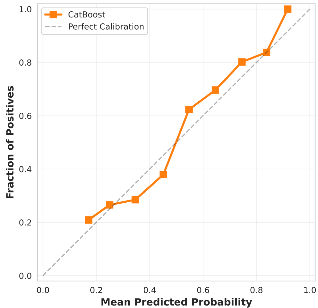
CatBoost (Brier Score = 0.2040)
