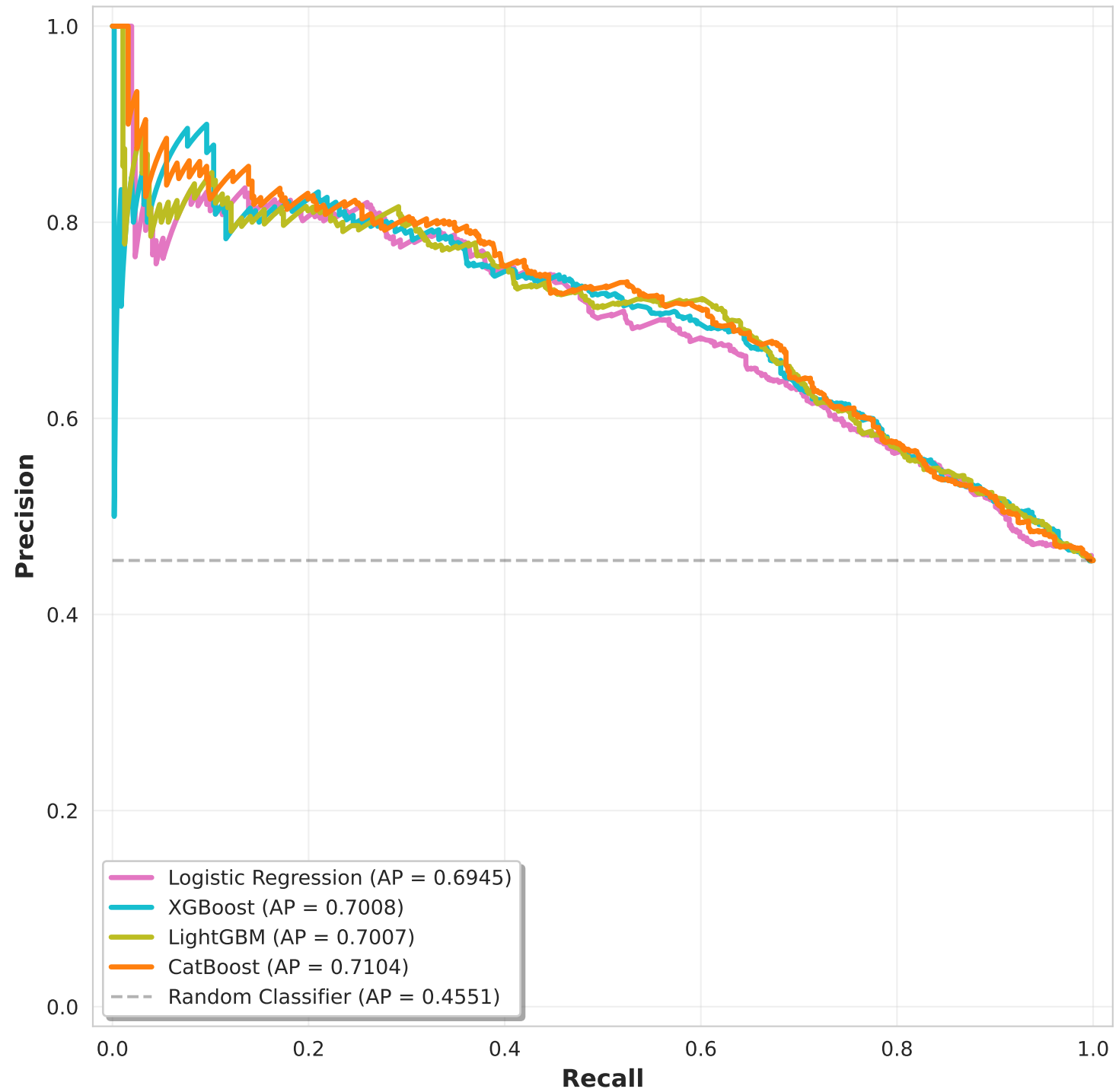
Precision-Recall Curves: COMPAS Recidivism Prediction
