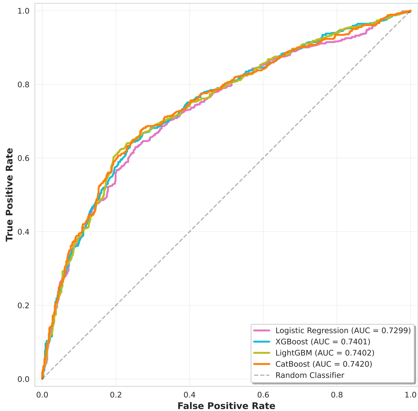
ROC Curves: COMPAS Recidivism Prediction
