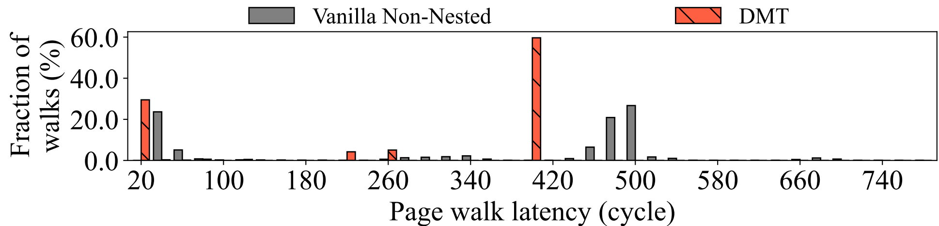
(b) Page walk latency distribution of Redis under non-nested environment
