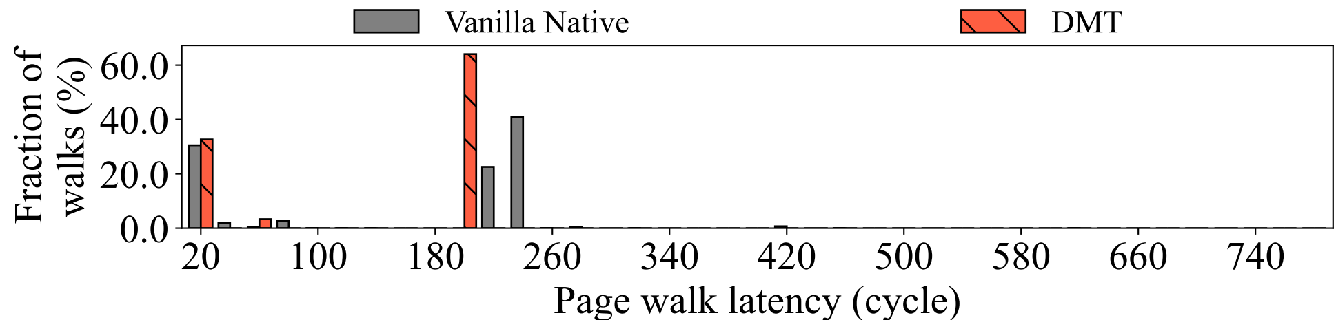
(a) Page walk latency distribution of Redis under native environment
