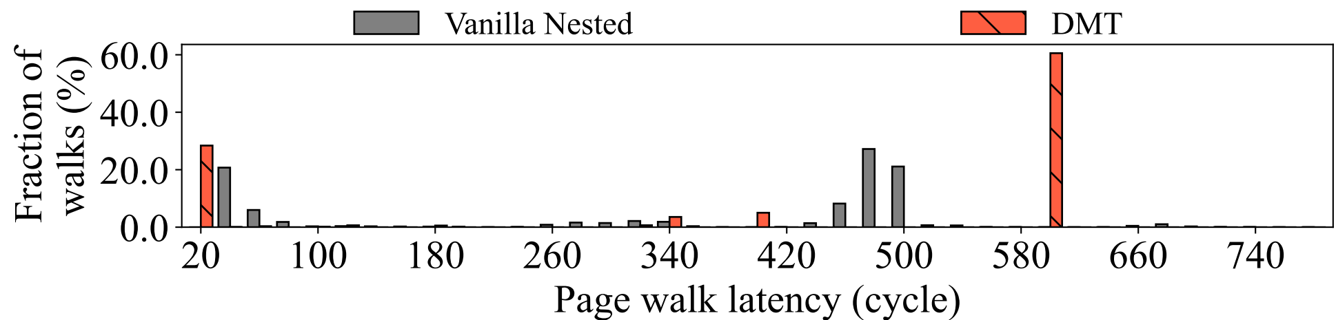
(c) Page walk latency distribution of Redis under nested environment
