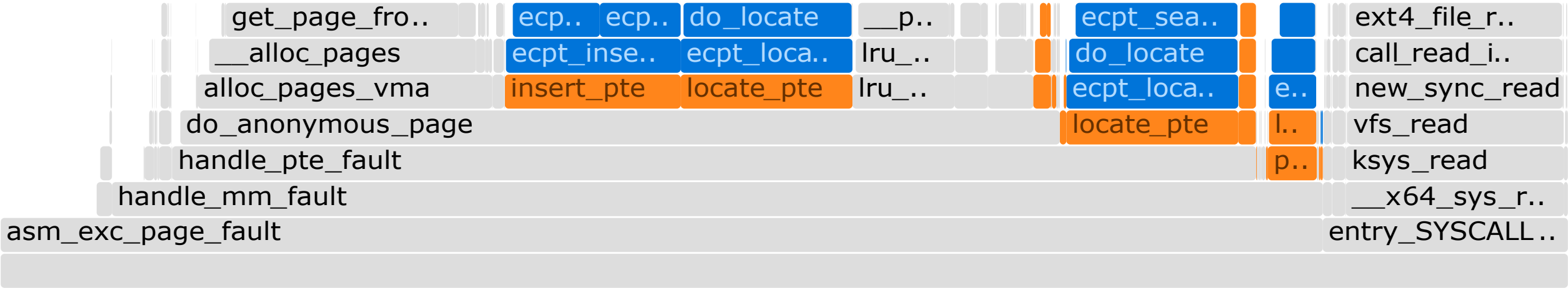
b) Kernel instruction flamegraph for 4KB of EMT-ECPT for graphbig_BFS
