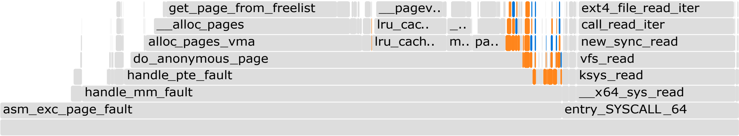
a) Kernel instruction flamegraph for 4KB of EMT-Radix for graphbig_BFS
