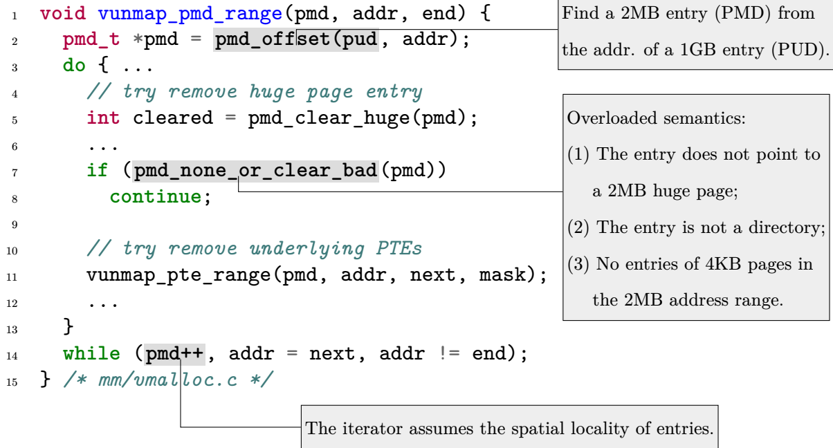
Figure 3: Examples of Linux memory management code that is hardcoded to radix-tree based translation.
