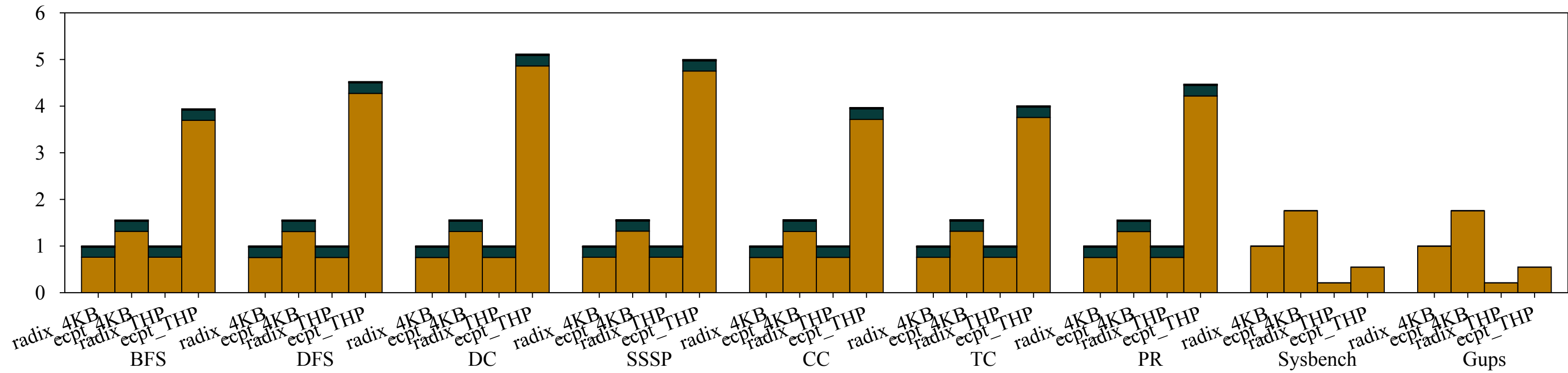
Kernel Instructions Breakdown
