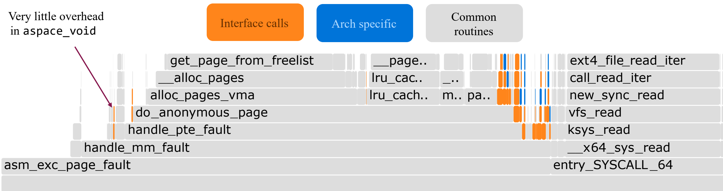
a) Kernel instruction flamegraph for THP of EMT-Radix for graphbig_BFS
