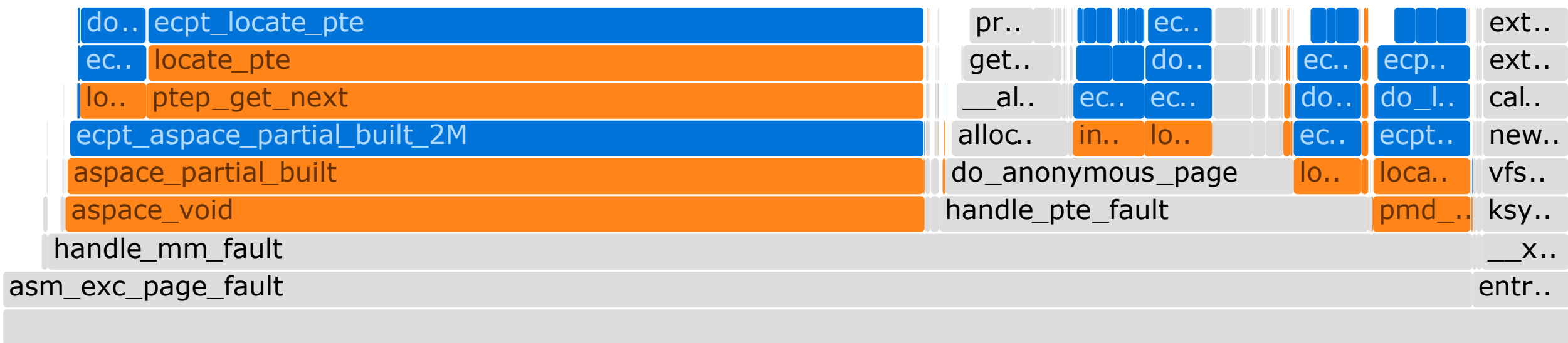
b) Kernel instruction flamegraph for THP of EMT-ECPT for graphbig_BFS
