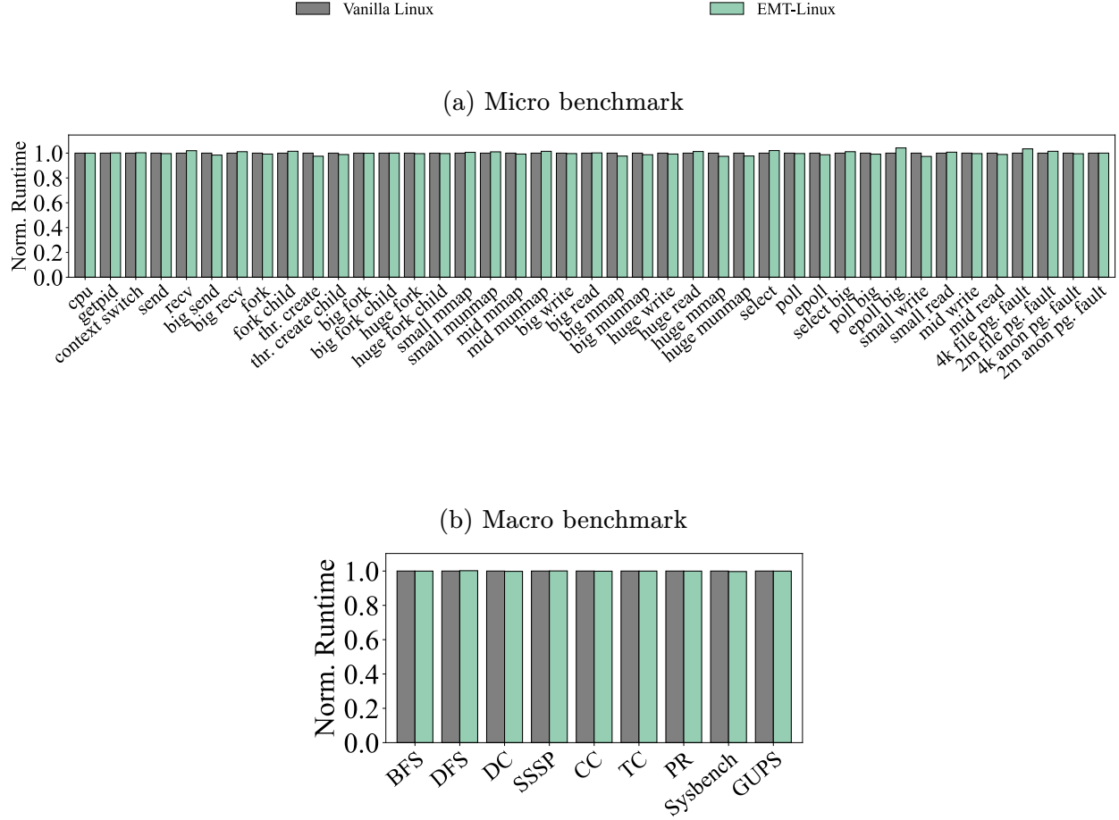
Figure 14: Performance overhead of EMT-Linux over vanilla Linux (measured by the micro and macro benchmarks).
