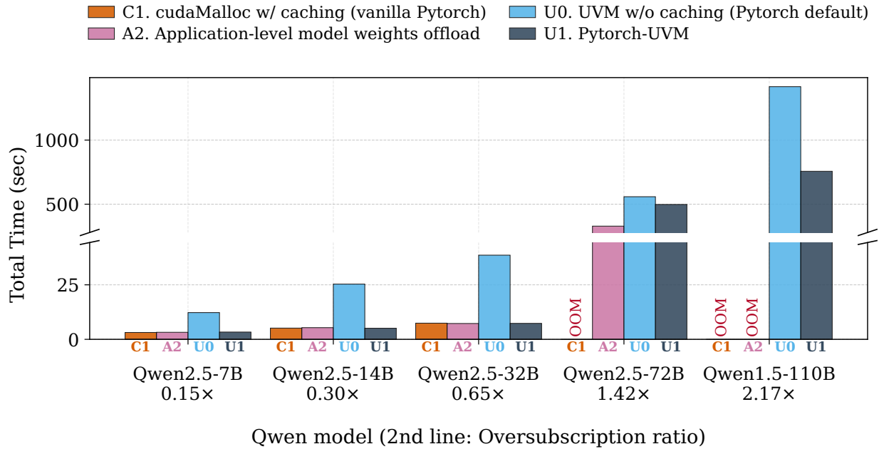
(b) Qwen models
