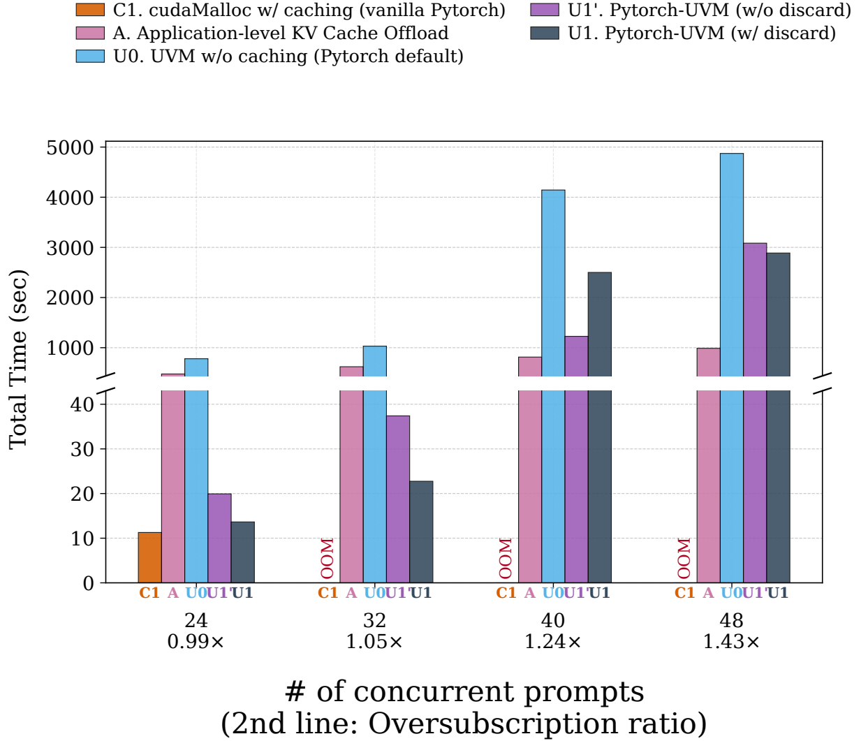
Figure 39: Effect of framework-guided eviction on H100 PCIe (4 KiB pages): total run time of OPT-13B for batch sizes spanning the oversubscription transition. U1 enables framework-guided eviction (implemented via UVMDiscard); U1' keeps the rest of PyTorch-UVM but evicts via copy-back to host. Reserved / active oversubscription ratios are bsz=24: 0.99\times / 0.81\times , bsz=32: 1.05\times / 0.97\times , bsz=40: 1.24\times / 1.14\times , bsz=48: 1.43\times / 1.31\times .
