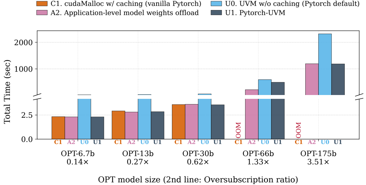
(a) OPT models
