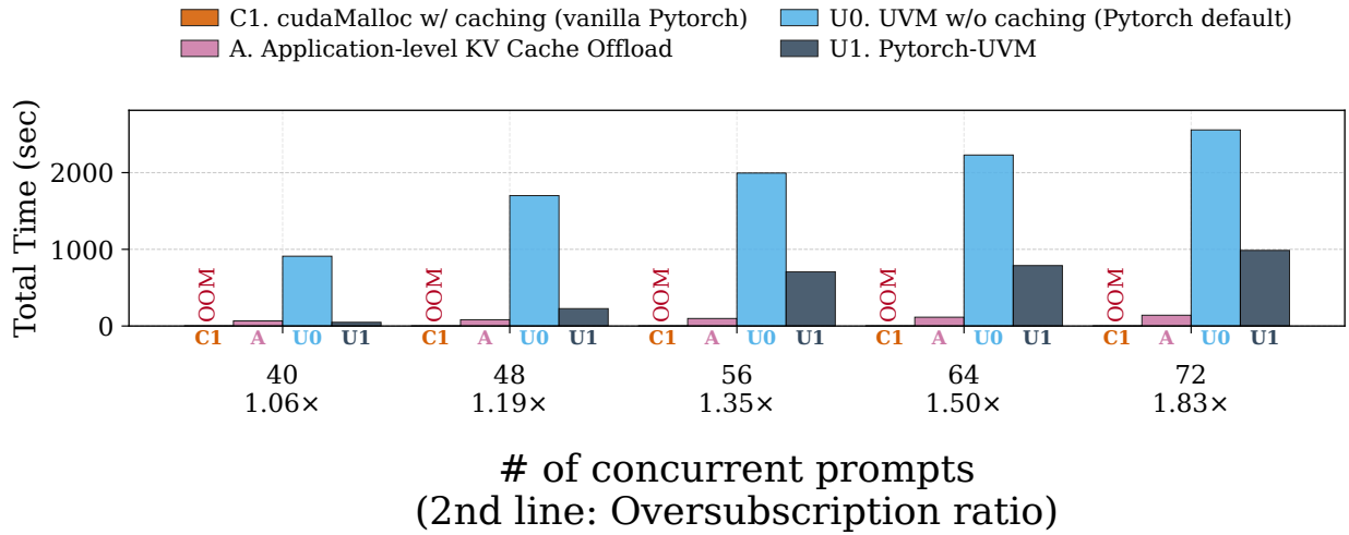
(b) Performance after oversubscription (batch size 40–72)
