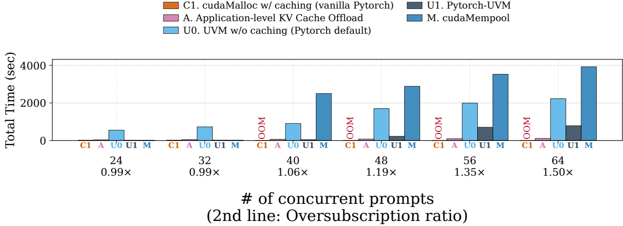
Figure 43: Comparison of PyTorch-UVM (U1) and a cudaMempool-based allocator (M) on GH200 NVLink-C2C, OPT-13B, batch sizes 24–64 ( 0.99\times – 1.50\times reserved oversubscription). Both allocators sit on top of cudaMallocManaged ; baselines C1, A, and U0 are shown for reference. At bsz 72 ( 1.83\times ) cudaMempool fails with a host-side OOM and is therefore omitted from the rightmost point.
