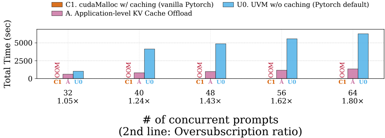
(b) With oversubscription
