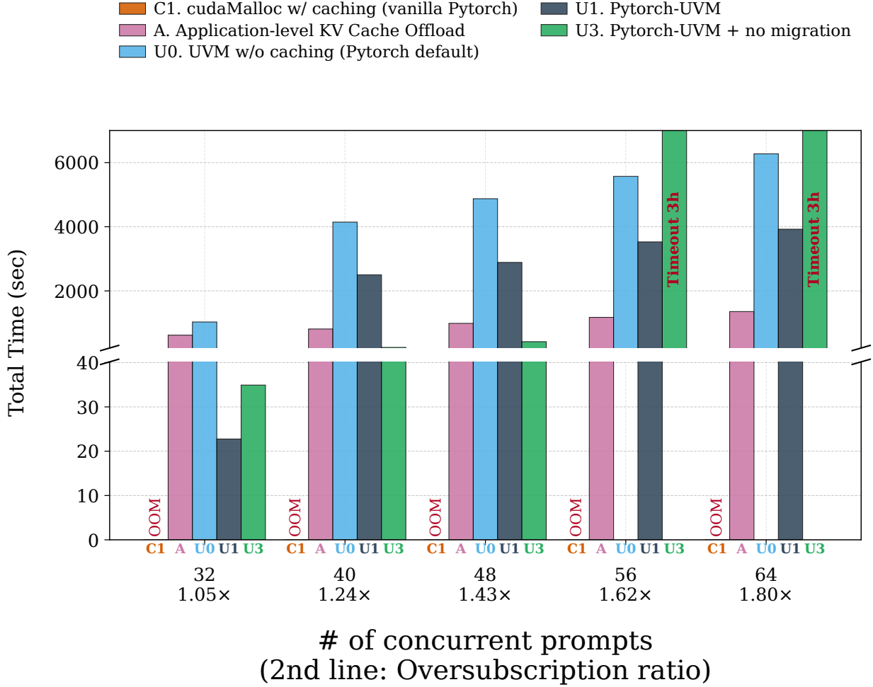
Figure 41: Effect of disabling migration on H100 PCIe (4 KiB pages): total run time of OPT-13B for batch sizes 32–64. U1 is PyTorch-UVM with on-demand migration; U3 is the same configuration with migration disabled, so that pages are accessed in place over PCIe (zero-copy). Reserved / active oversubscription ratios are bsz=32: 1.05\times / 0.97\times , bsz=40: 1.24\times / 1.14\times , bsz=48: 1.43\times / 1.31\times , bsz=56: 1.62\times / 1.48\times , bsz=64: 1.80\times / 1.65\times . Bars at 10,800s indicate runs that hit the 3-hour timeout.
