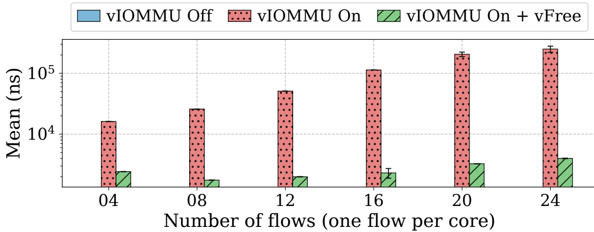
(c) IR processing latency per unmap
