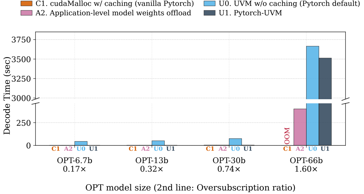
(a) OPT models (decode time)
