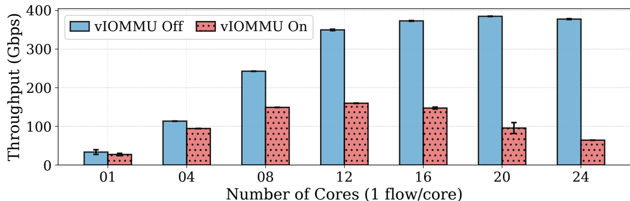
(b) Rx-server (VM running as a receiver)
