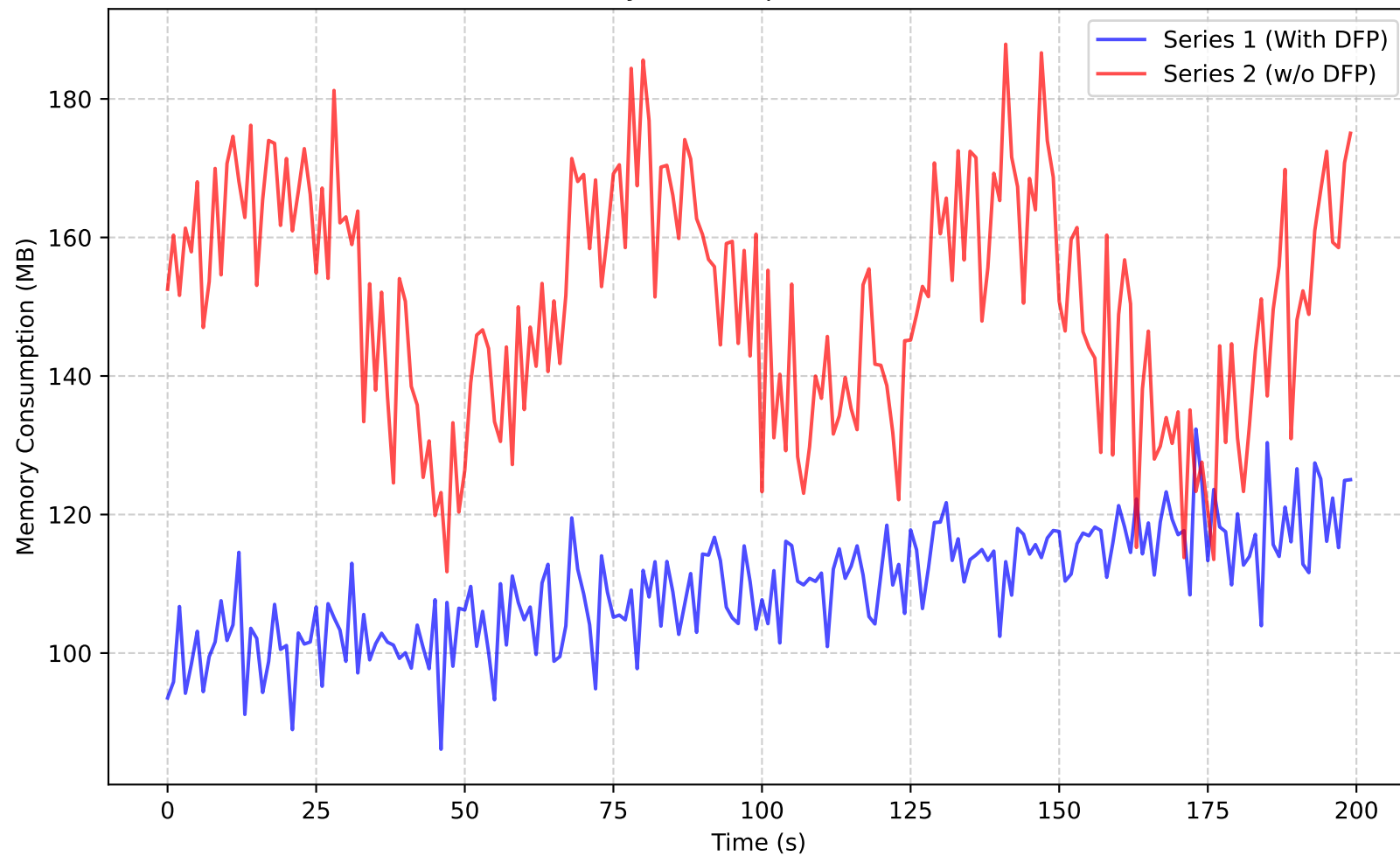
Memory Consumption Over Time
