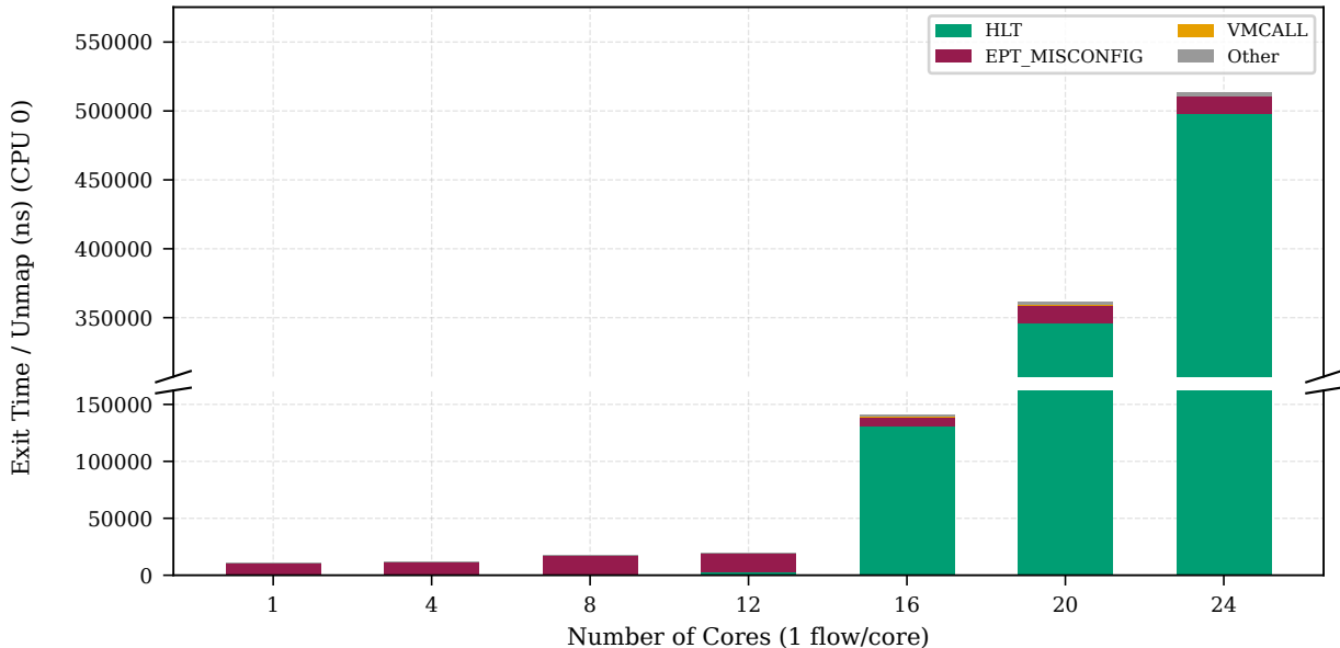
VM Exit Time per Unmap Call by Type
