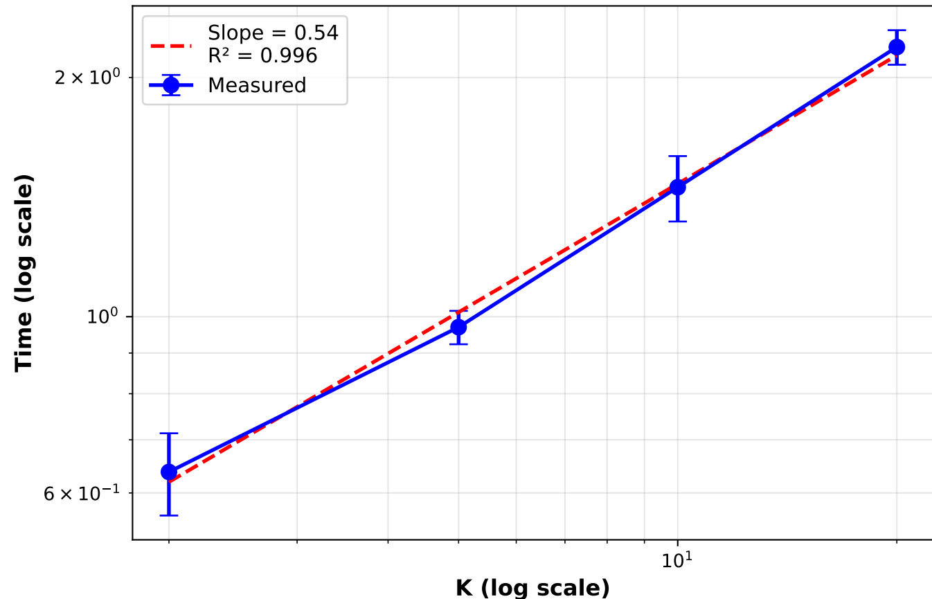
Log-Log Plot (Slope = Complexity Exponent)
