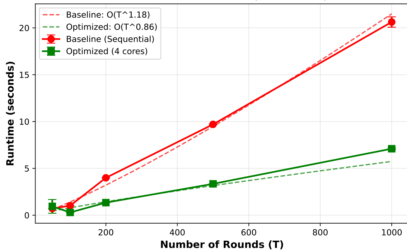
Runtime vs Problem Size (Linear Scale)
