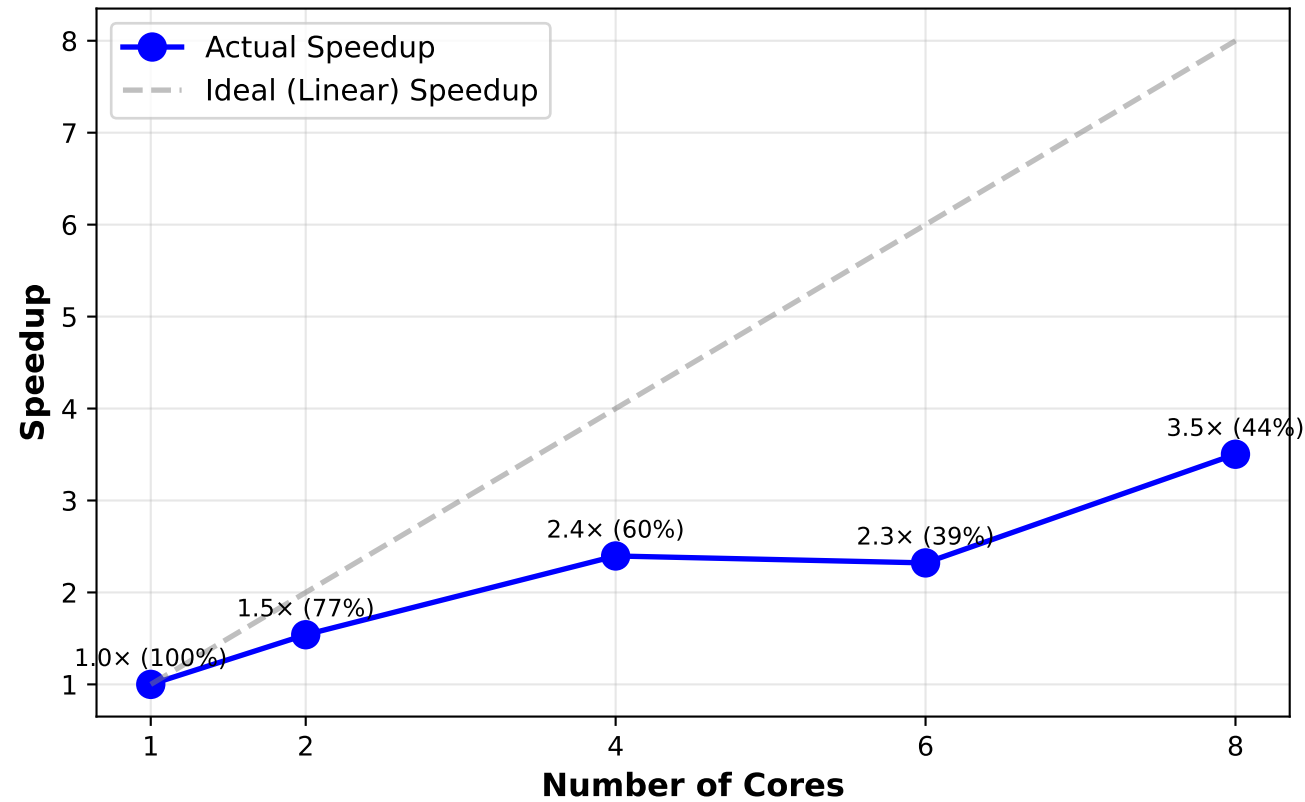
Speedup vs Number of Cores
