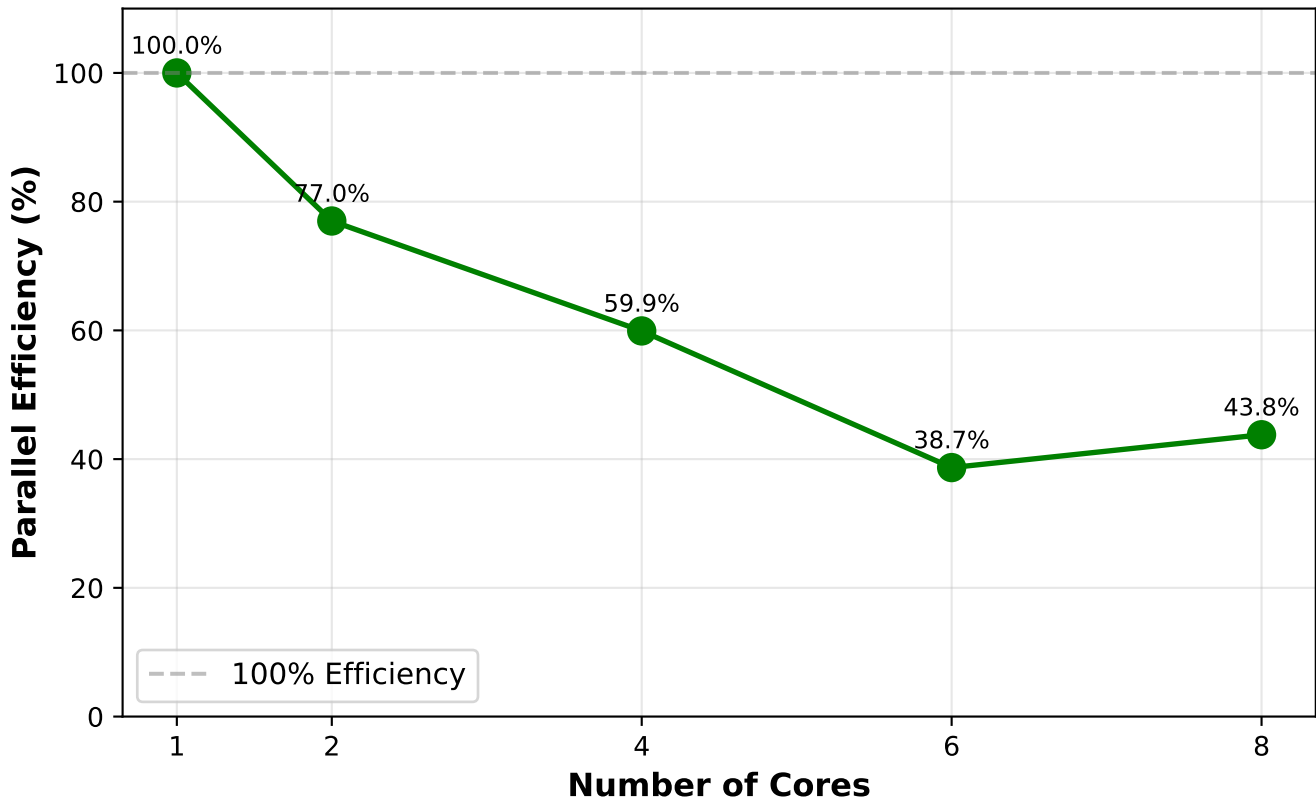
Parallel Efficiency
