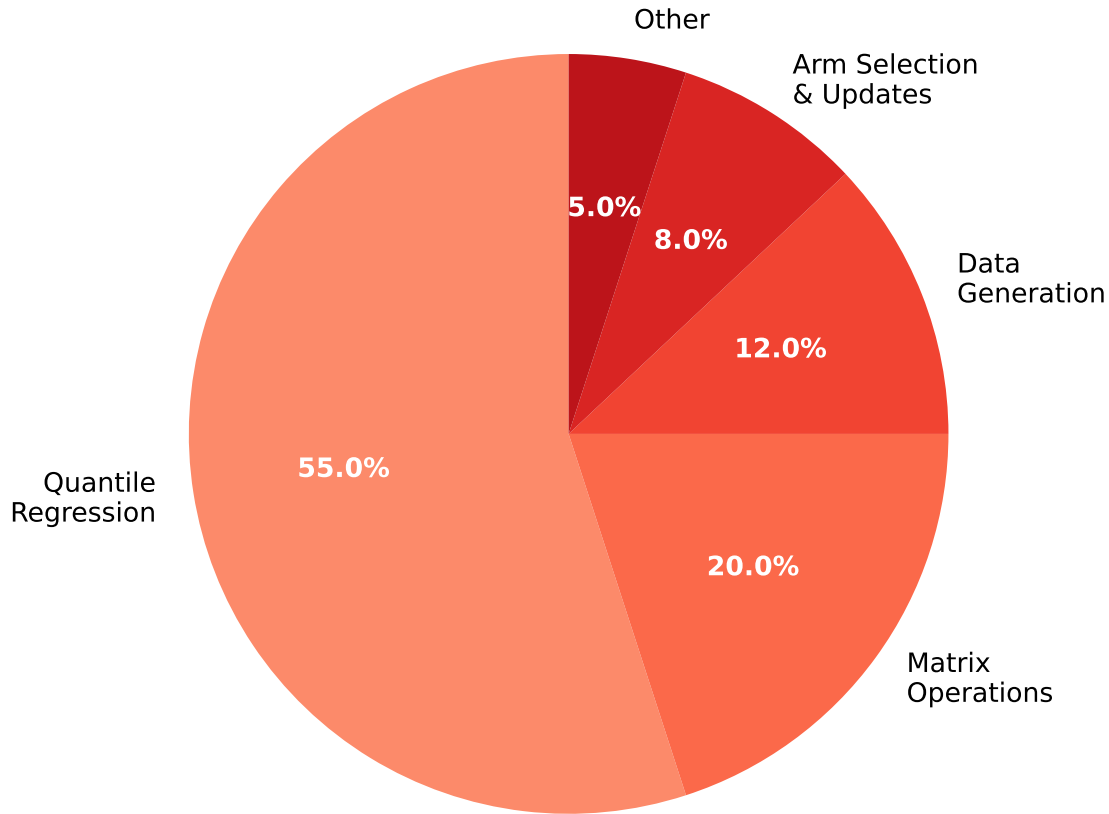
Baseline (Sequential) Time Breakdown
