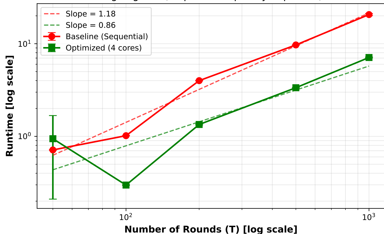
Log-Log Plot (Slope = Complexity Exponent)
