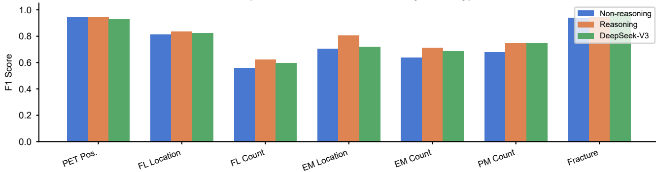
Task-specific Extraction Performance by Model Type
