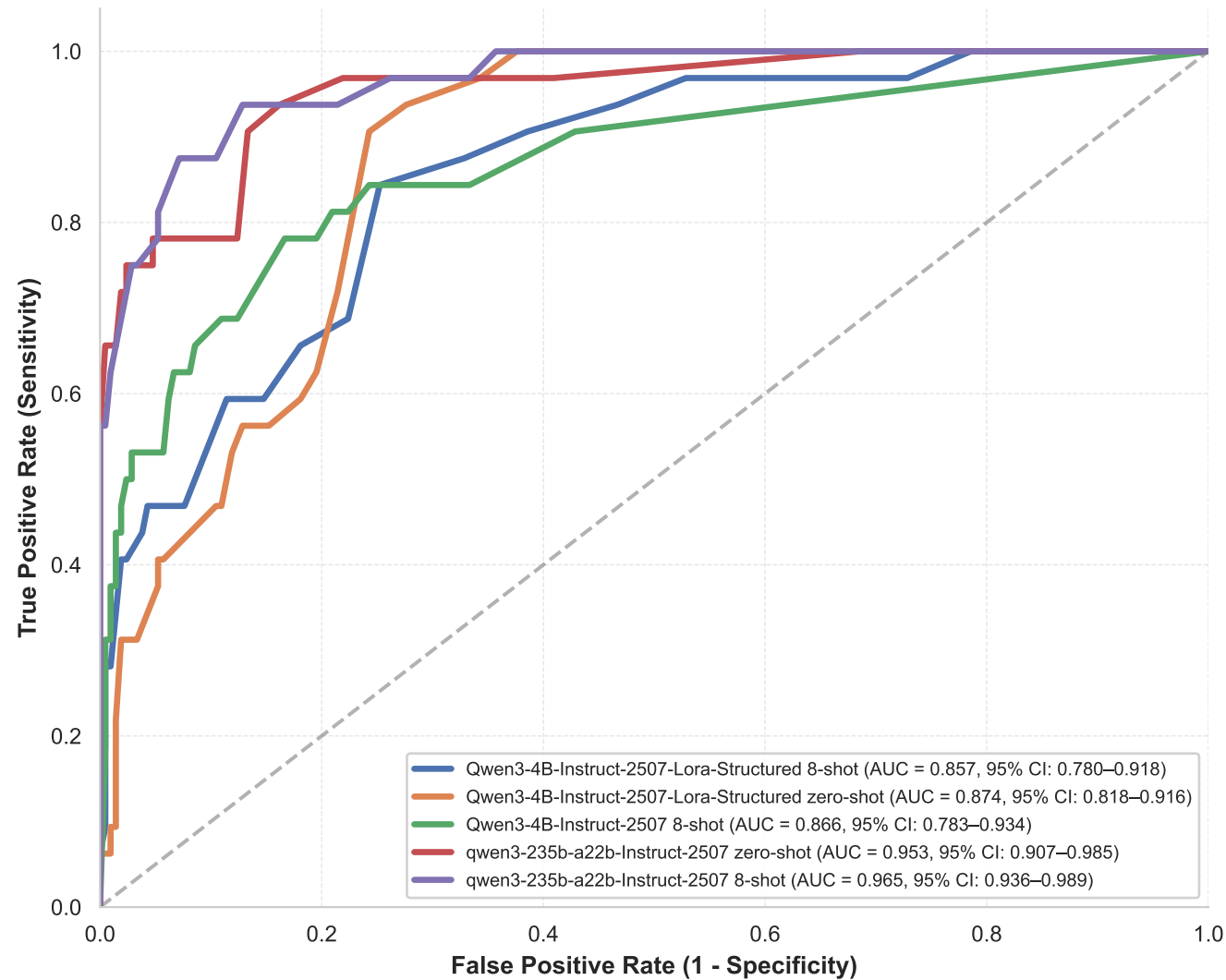
A | ROC Curve Comparison
