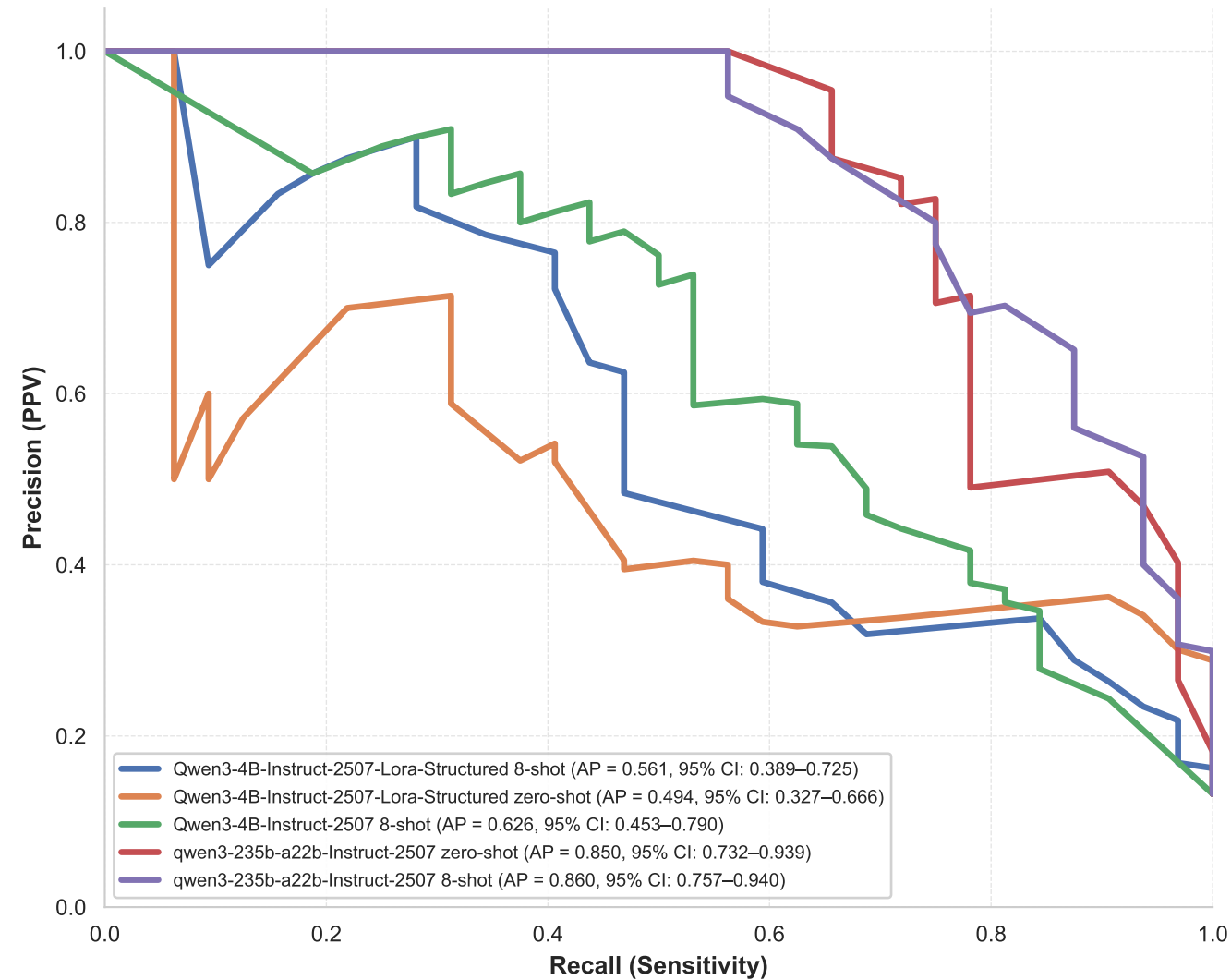
B | Precision-Recall Curve Comparison
