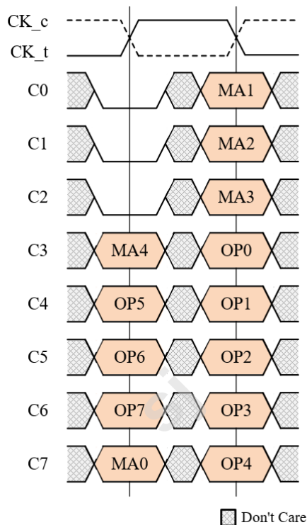
Figure 49 — Mode Register Set Command (MRS)
