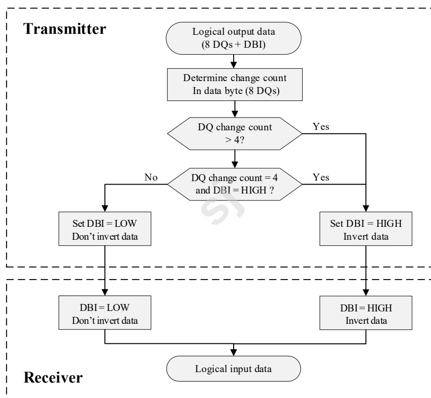
Figure 13 — DBIac Algorithm
