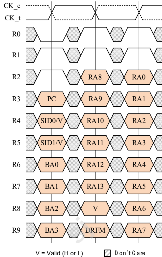
Figure 18 — ACTIVATE Command
