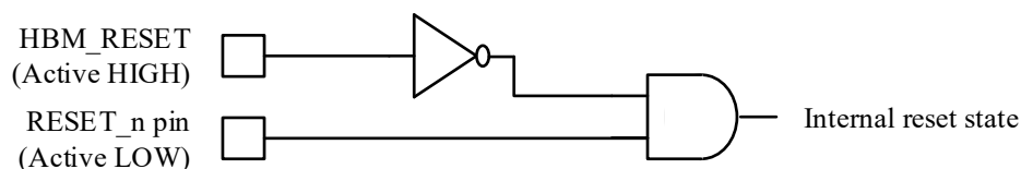
Figure 114 — RESET_n and HBM_RESET Logic
