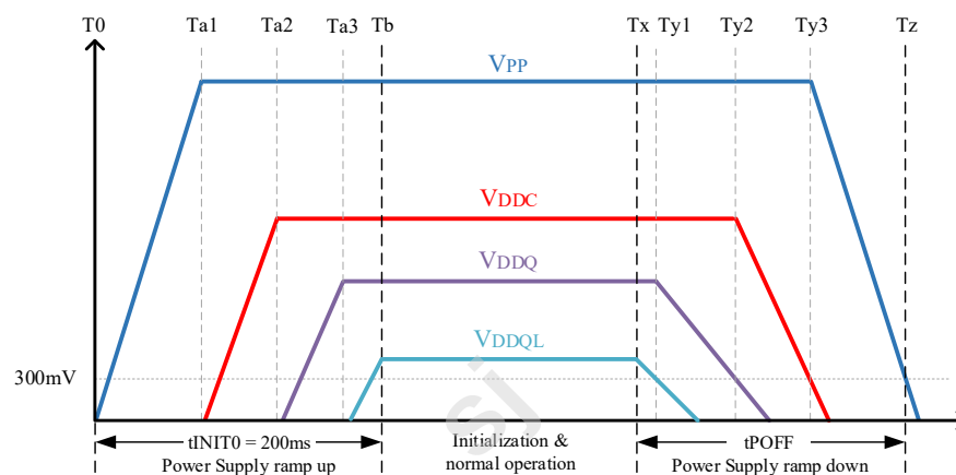
Figure 4 — Recommended Power-up and Controlled Power-off Sequence
