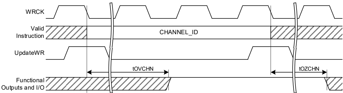
Figure 124 — IEEE1500 CHANNEL_ID Instruction Related Timings
