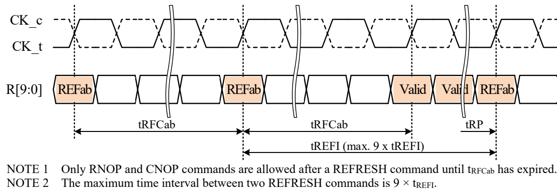
Figure 24 — REFab Cycle
