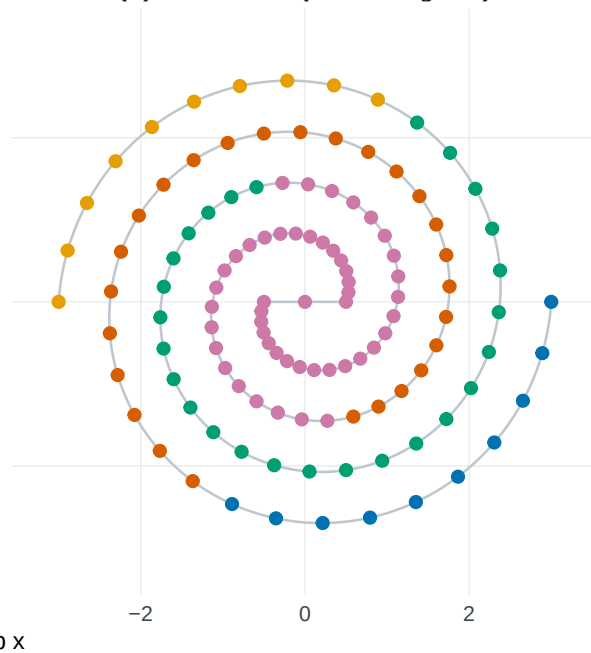
(b) Recovered partition (joint)
