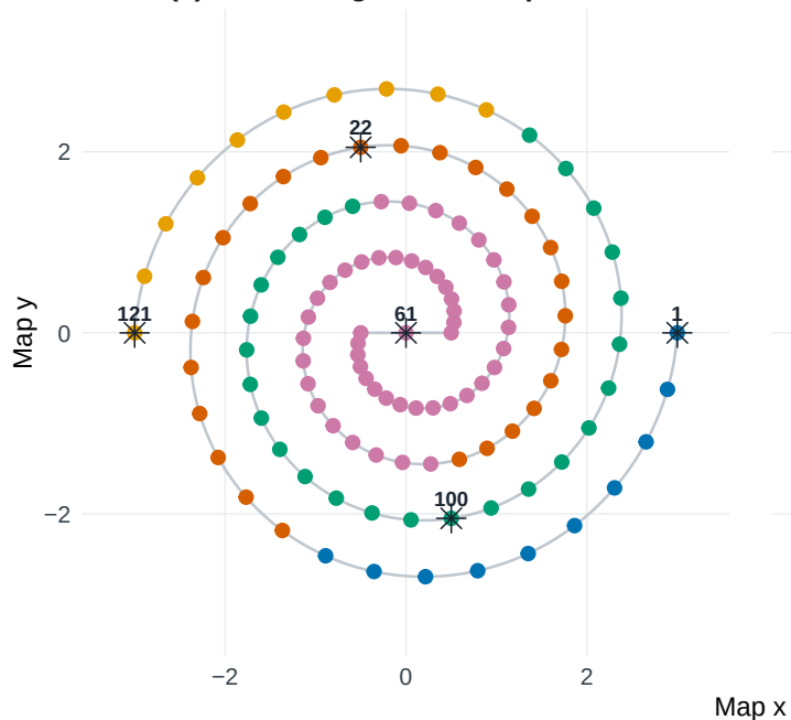
(a) Generating five-class partition
