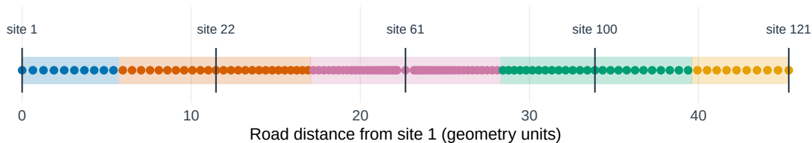
(c) The same road unfolded; boundaries are nearest-seed midpoints
