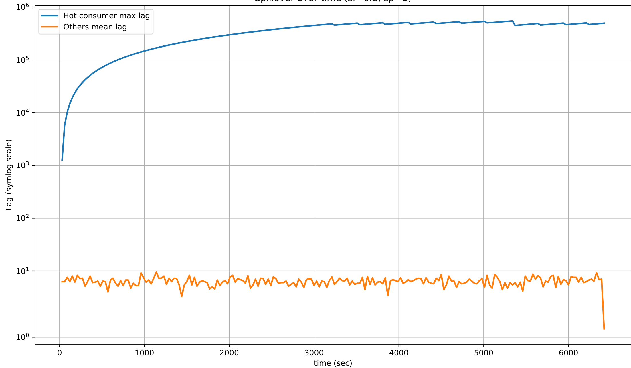
Spillover over time (sf=0.8, sp=0)
