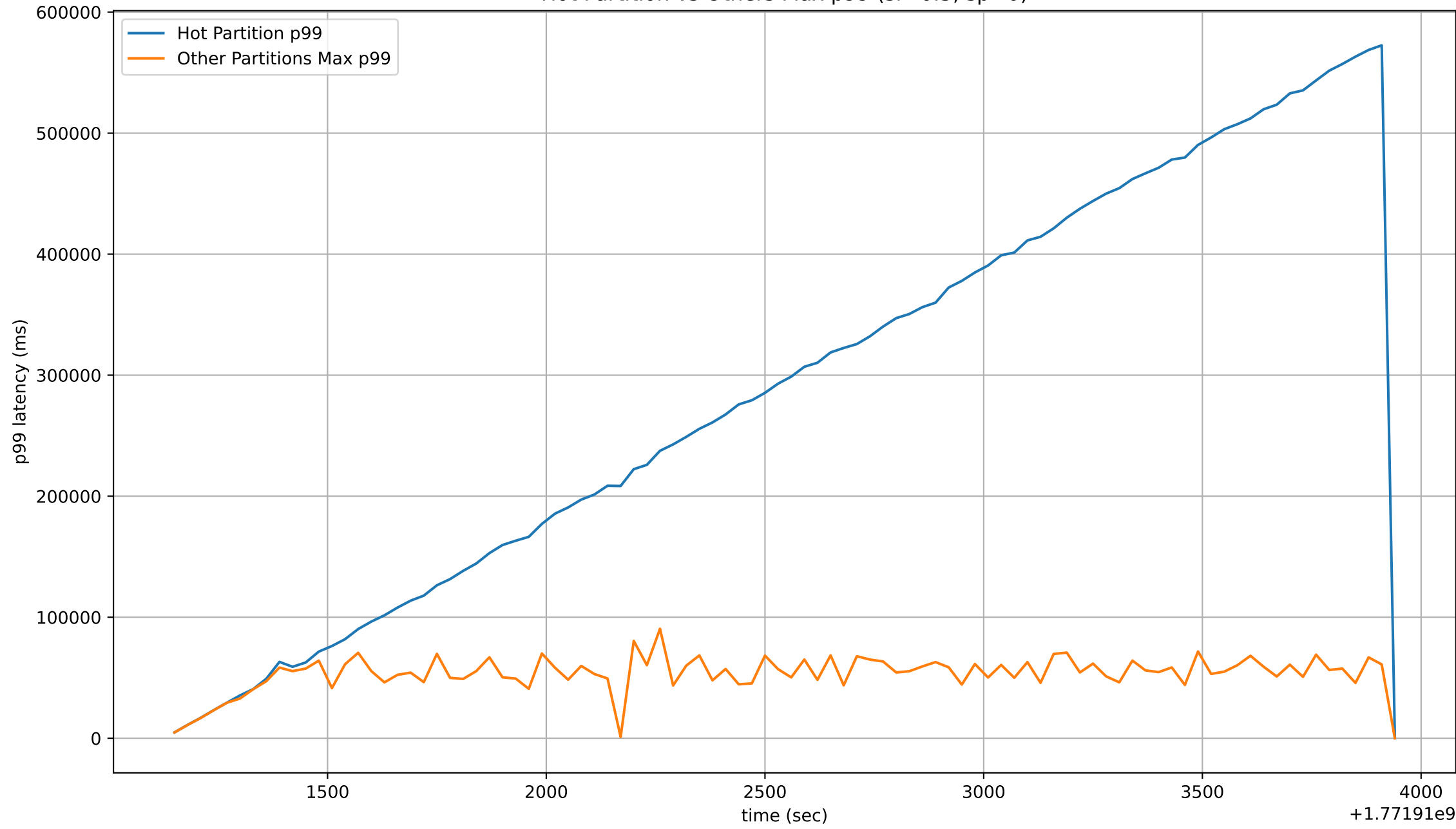
Hot Partition vs Others Max p99 (sf=0.3, sp=0)
