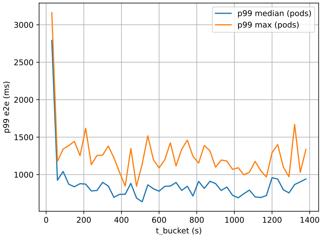
p99 latency (tm=balanced, sf=0.0166, sp=0)
