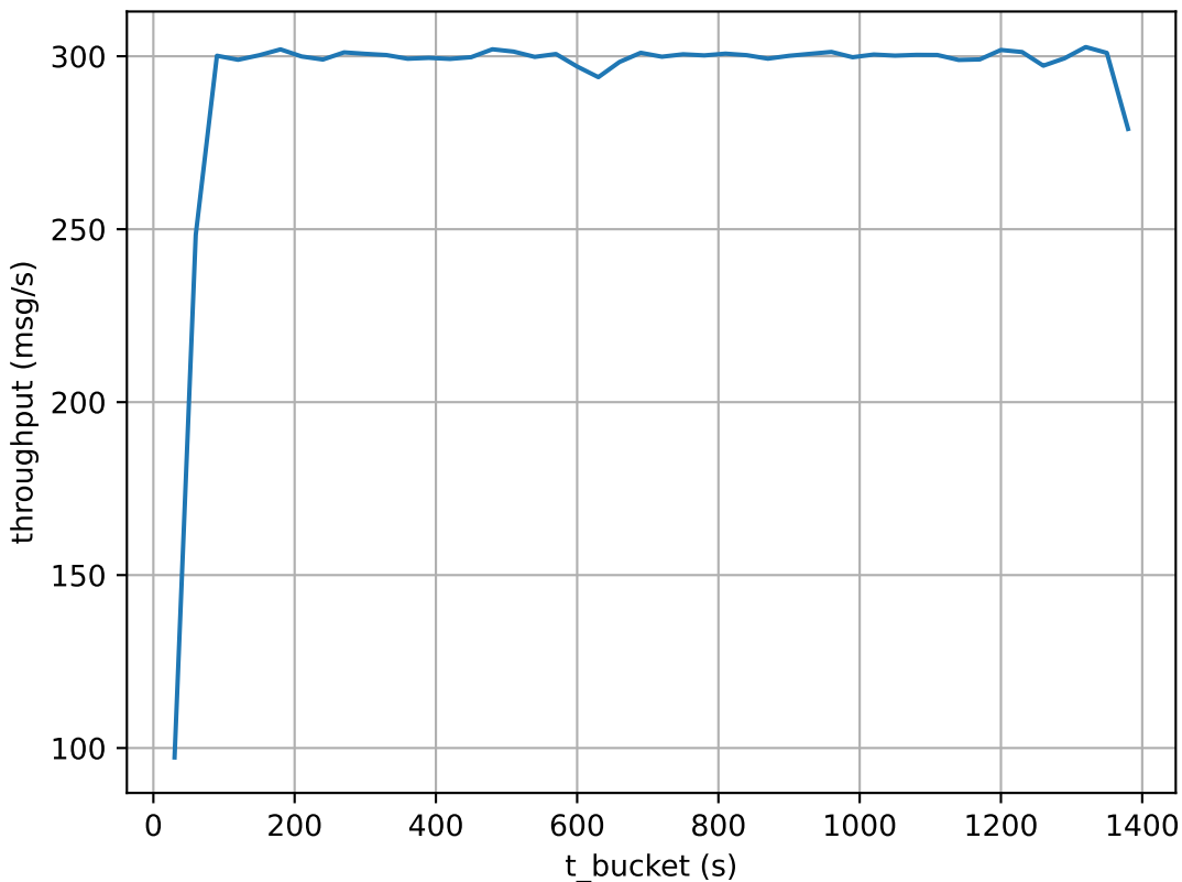
Throughput (tm=balanced, sf=na, sp=unknown)
