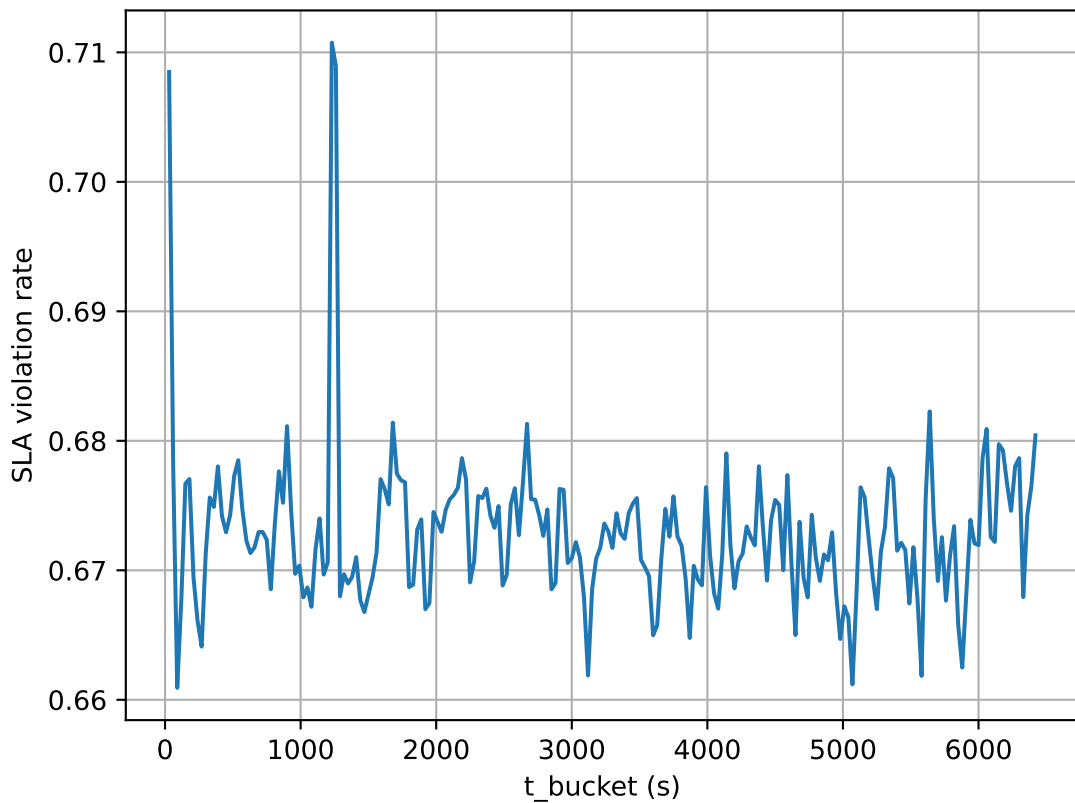
SLA violation (tm=skew, sf=0.8, sp=0)
