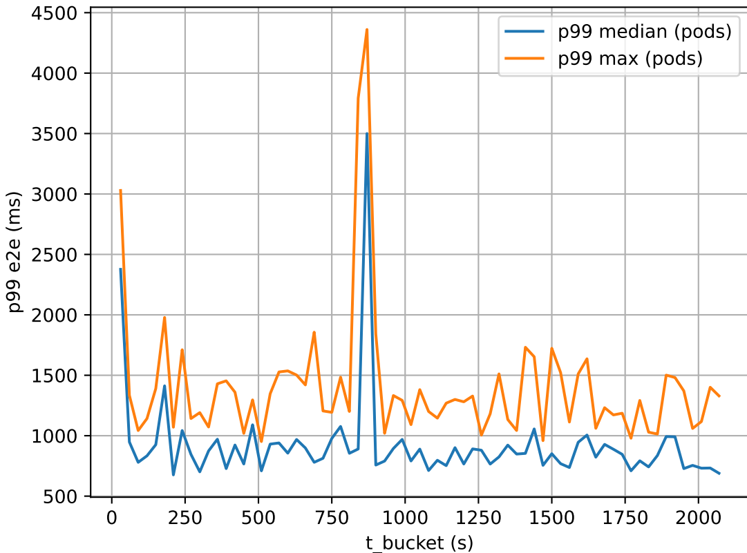
p99 latency (tm=skew, sf=0.05, sp=0)
