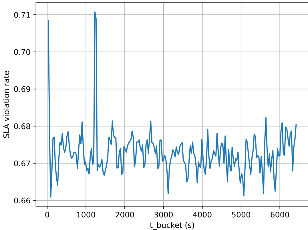
SLA violation (tm=skew, sf=0.5, sp=0)
