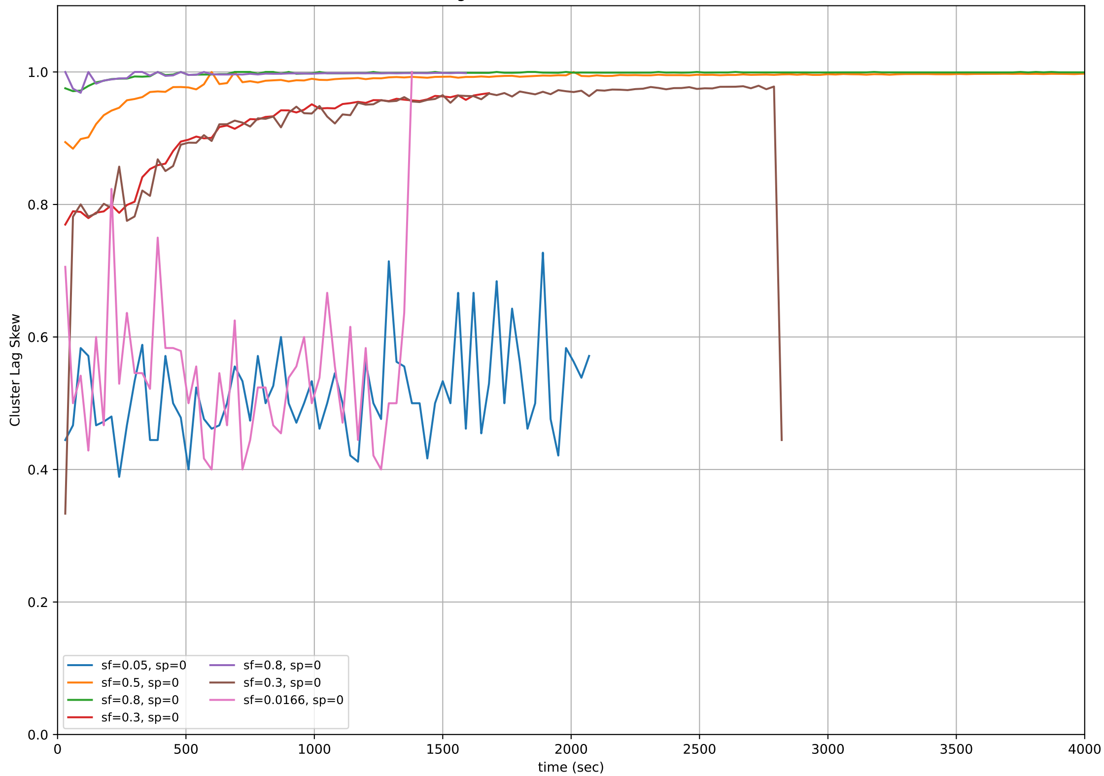
Lag Skew Over Time for All Runs.
