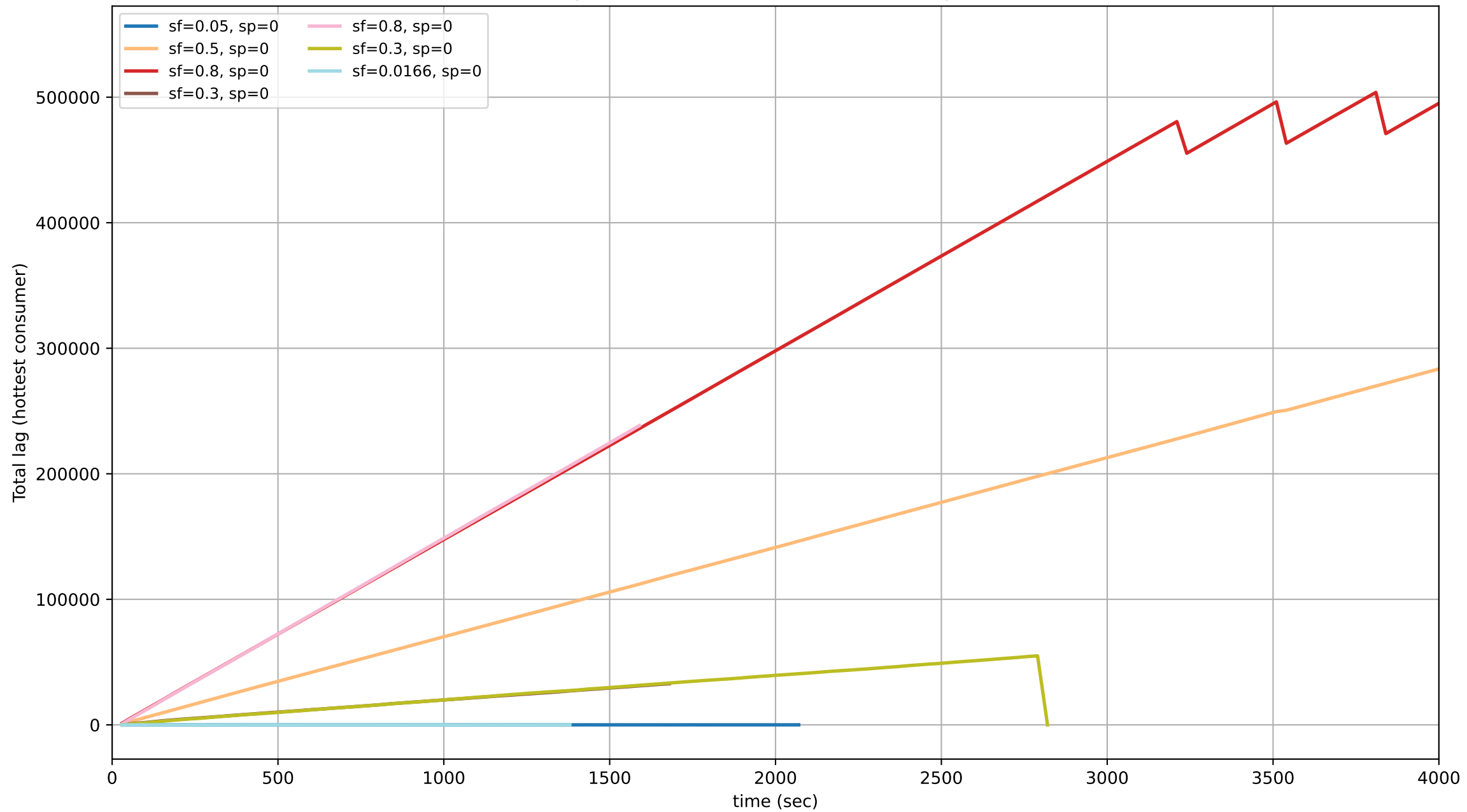
Total Lag of Consumer with Max Partition Lag (All Runs)
