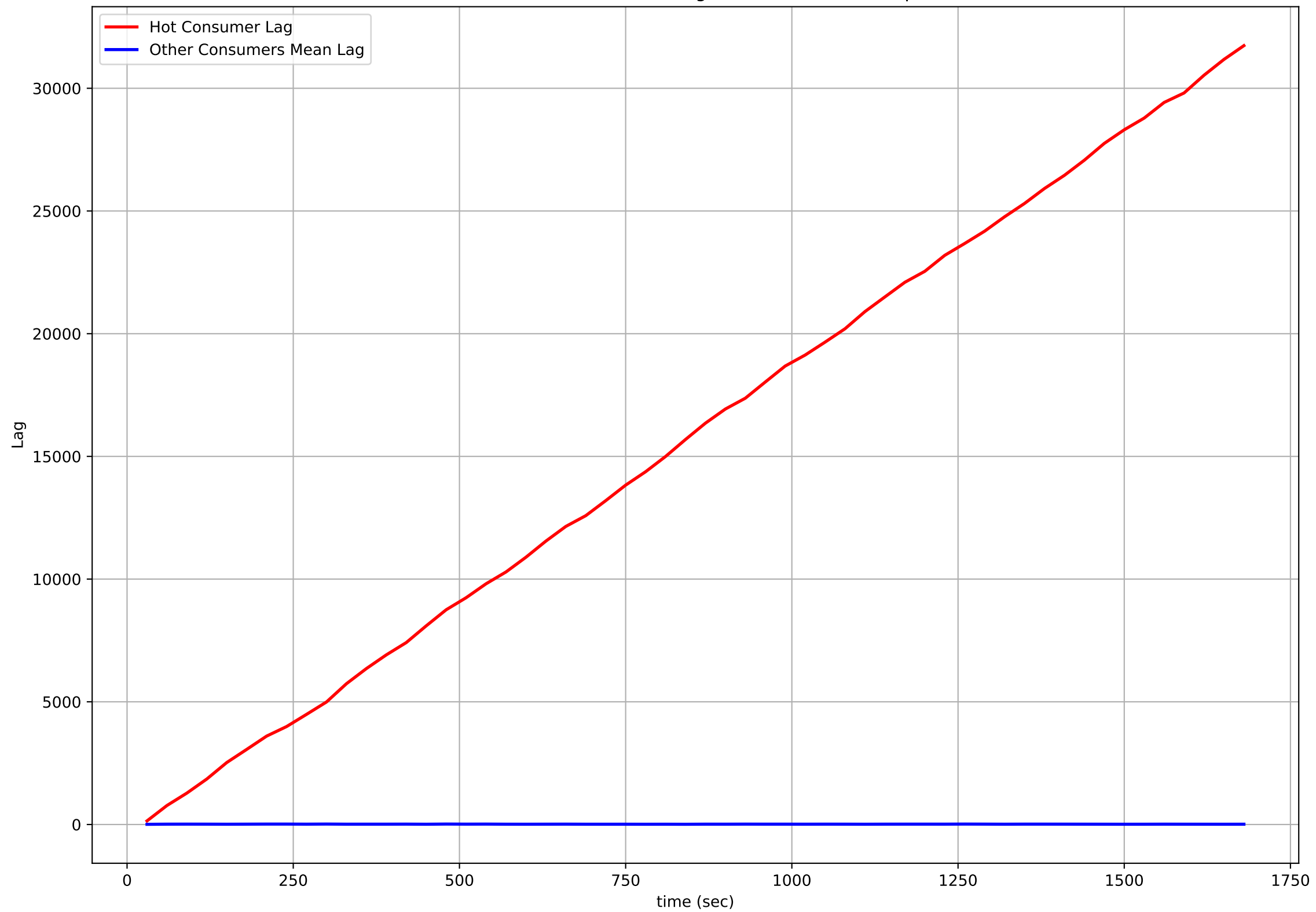
Hot Consumer vs Others Lag Over Time (sf=0.3, sp=0)
