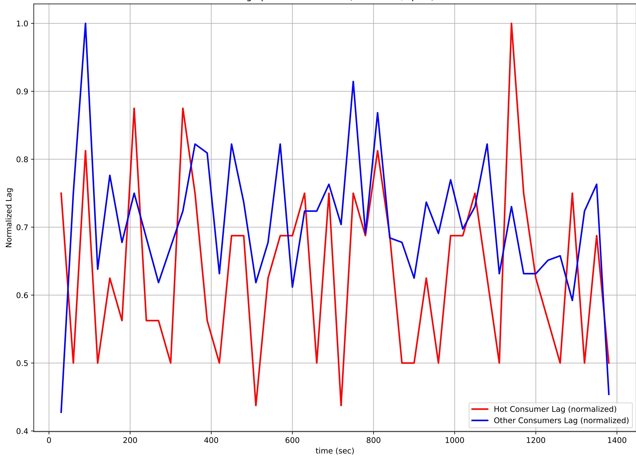
Lag Spillover Over Time (sf=0.0166, sp=0)
