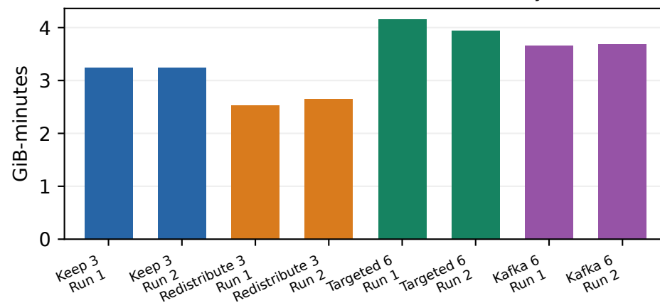
Observed consumer resident memory
