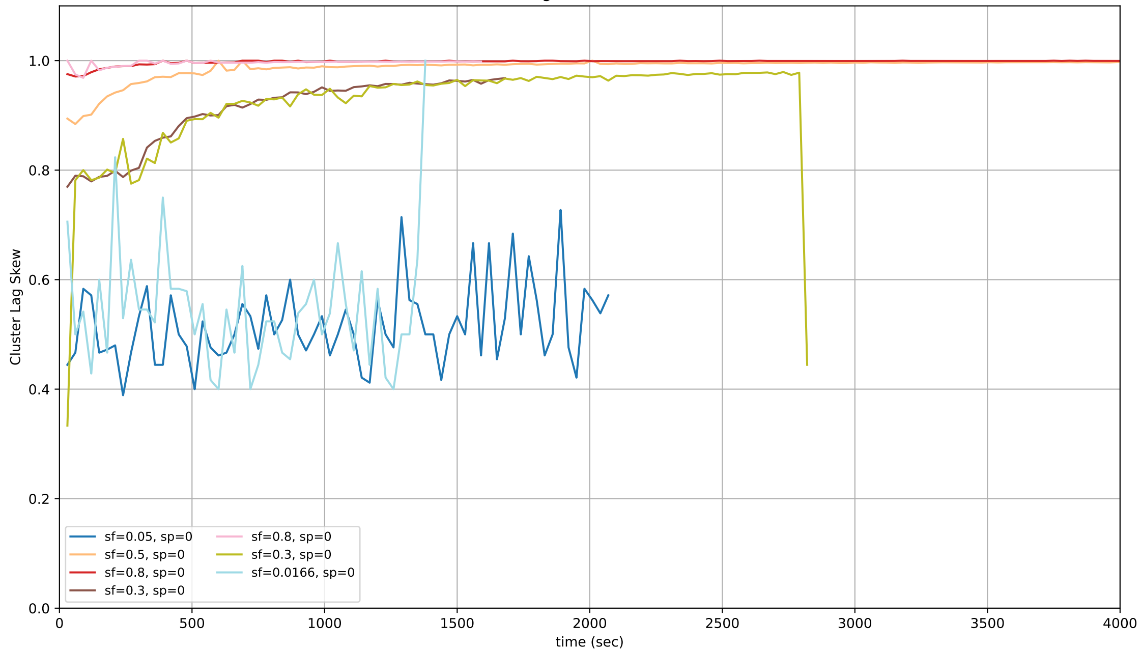
Max Consumers Lag Skew Over Time for All Runs.
