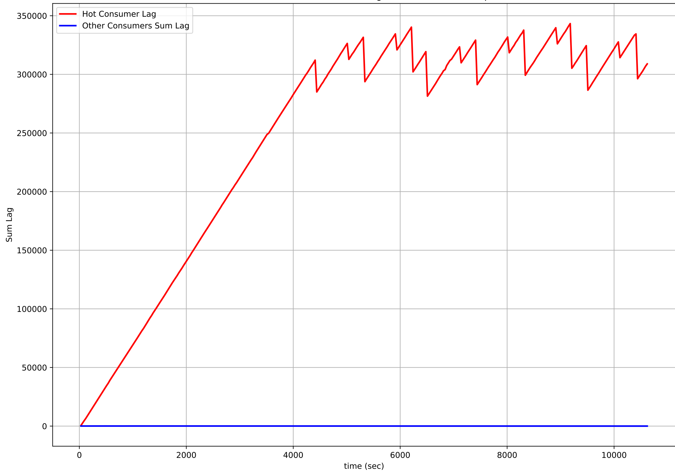
Hot Consumer vs Others Sum Lag Over Time (sf=0.5, sp=0)
