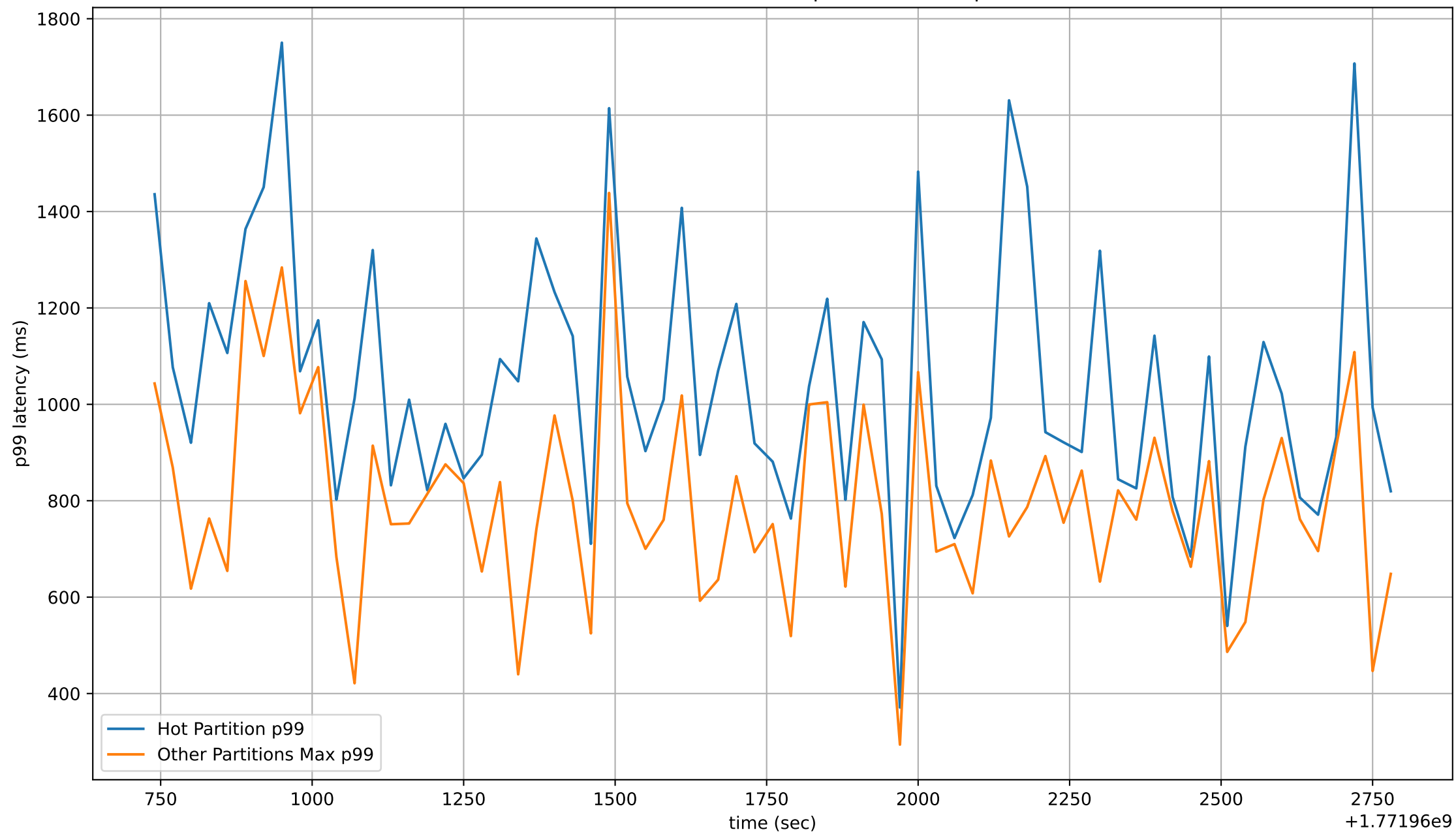
Hot Partition vs Others Max p99 (sf=0.05, sp=0)
