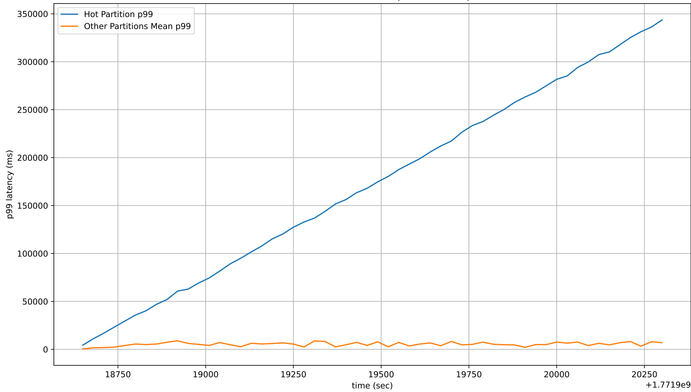
Hot Partition vs Others Mean p99 (sf=0.3, sp=0)
