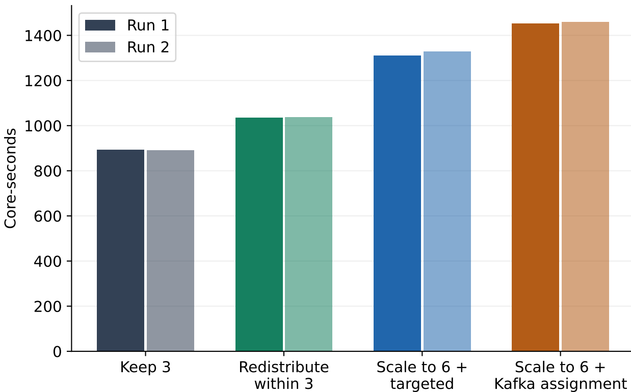
Measured consumer CPU time
