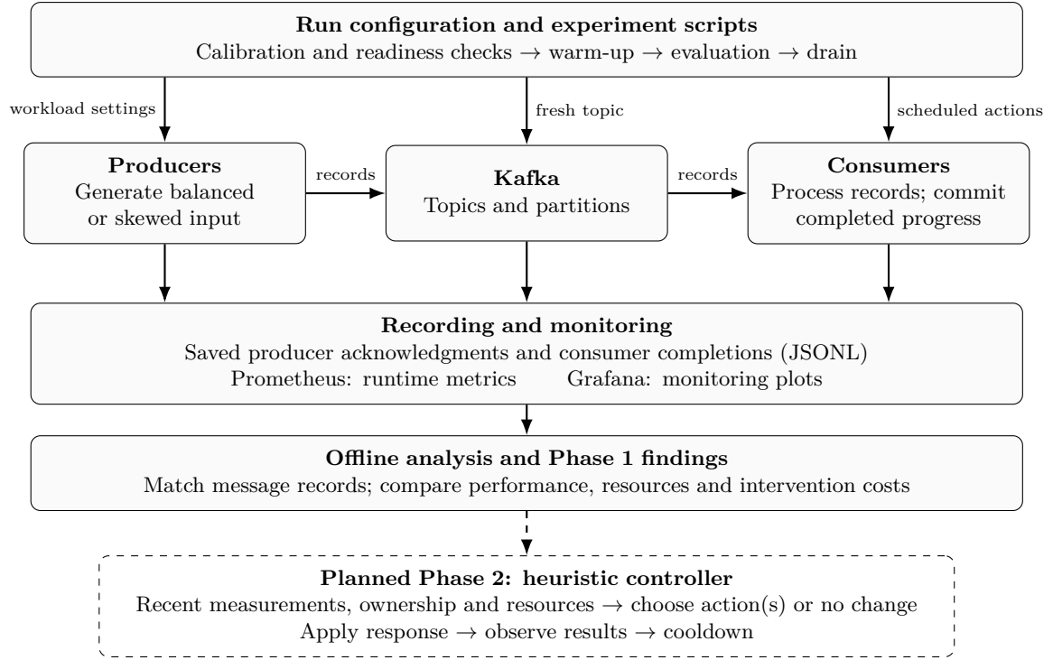
Figure 1: System architecture and experimental workflow. Solid boxes show the current pipeline and experiment procedure. The dashed box shows the planned controller, which will coordinate consumer scaling, partition reassignment or permitted hot-key splitting. The current trials use scheduled actions.
