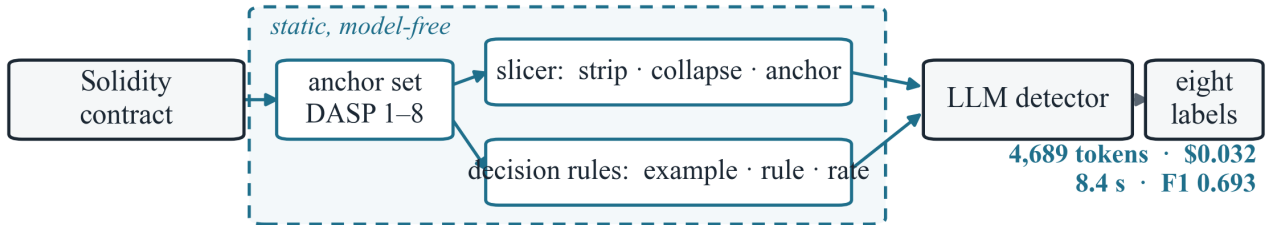
FIGURE 1: AnchorSlice and the practice it replaces. Conventionally the whole contract is handed to the detector with a one-line list of the categories. AnchorSlice derives two static components from one anchor set per DASP category: a slicer, which emits a tagged slice of 56.5% of the source characters while retaining all 463 labelled category instances, and a set of decision rules, which state what each category means in this corpus. The detector, Claude Opus 5, and the output schema are identical in both arms; figures beneath each lane are per contract.
