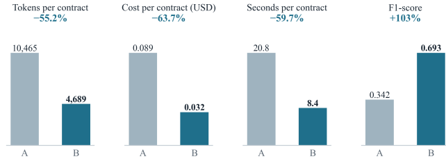
FIGURE 3: Resource use and detection quality per contract, Arm A against Arm B. Token consumption, cost and latency fall by more than half while F1-score doubles.
