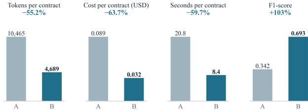
Fig. 3. Resource use and detection quality per contract. Tokens, cost and latency fall by more than half while F1-score doubles.
