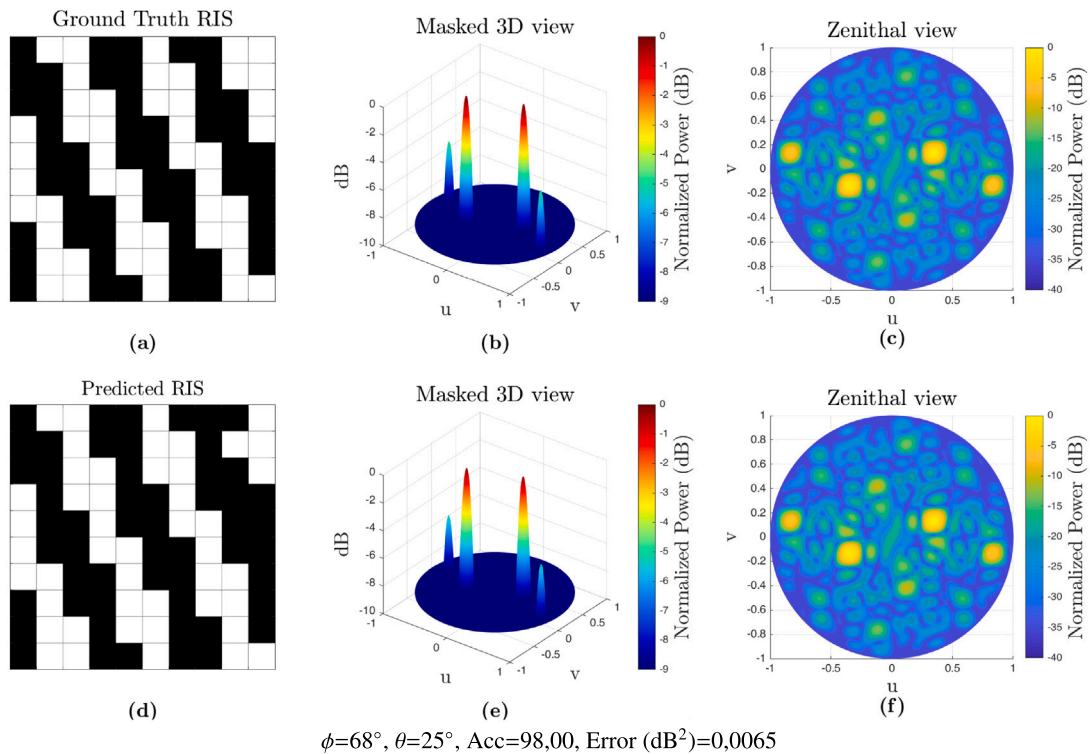
Fig. 4. Ground-truth and predicted 10 \times 10 RIS configurations for the \phi = 68^\circ , \theta = 25^\circ target angle alongside their corresponding radiation patterns. (a) and (d) show the ground-truth and the predicted RIS configurations (b) and (e) display 3D-views of the radiation patterns when a -9 dB mask is applied. (c) and (f) present zenithal views of the complete radiation patterns.
