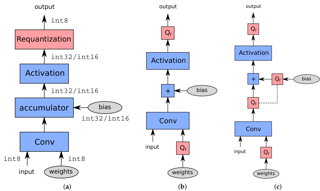
Figure 2. (a) Fixed-point compute engine of a convolutional layer; (b) simulated fixed-point compute engine with 32 bit accumulator and bias; (c) simulated compute engine with 16 bit (or less) accumulator and bias. The dashed line indicates that these fake quantization nodes share the same scale factor.
