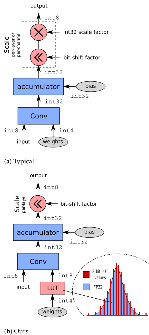
Figure 1. (a) Typical fixed-point compute engine of a convolutional layer; (b) our proposed fixed-point compute engine with a single per-layer power-of-two scale (bit-shift) and a lookup-table to translate 4 bit weights from storage to 8 bit weights for internal computation. The LUT is used to boost the expressive power of the engine through nonuniform weight quantization, which compensates the lack of high-precision scaling.
