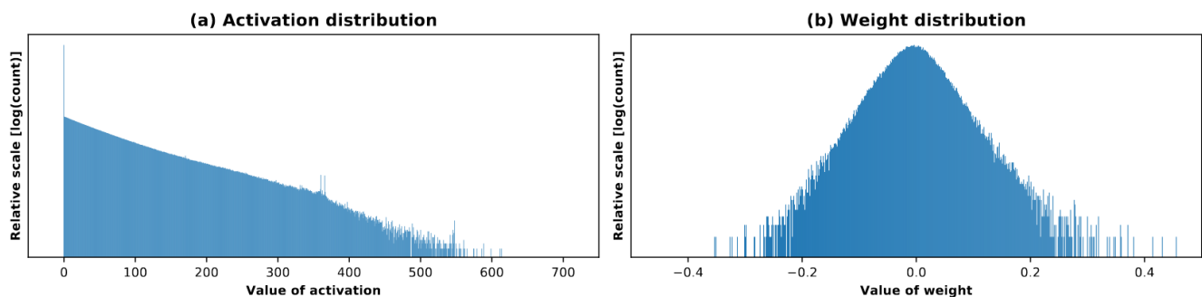
Figure 4. Activation and weight distribution of the second layer of GoogleNet (image from [27]).
