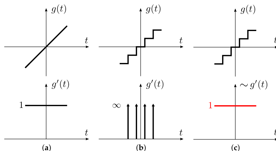
Figure 3. At the top, transfer functions of an identity function (a) and a round function (b) with their respective derivatives at the bottom. A round function with the STE in the backward pass is depicted in (c).
