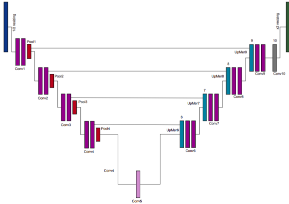
Figure 12. U-Net model proposed by MegaUe team.
