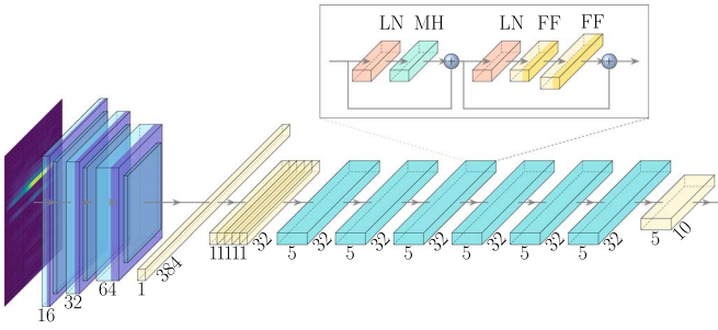
Fig. 7. Overall architecture of TR-former. The front end comprises 3 tokenizers blocks, each containing pointwise convolution, depthwise convolution, and pooling, followed by a linear layer. Each of the six encoder blocks consists of layer normalization layers (LN), a MHSA layer (MH), and linear layers (FF).
