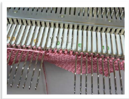
Needle L3 in hold to wrap Needles R4 .... In hold Needles L2 – R3 in work
