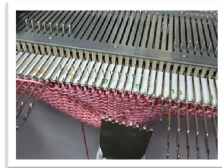
Automatic Wrap on carriage side 2 needles in working position opposite carriage
