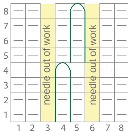
tuck stitch sequence (single repeat)
