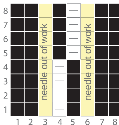
punchcard layout (single repeat)
