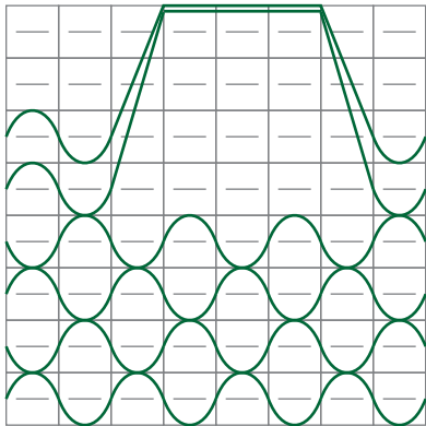
Weaving Sequence (single repeat)
