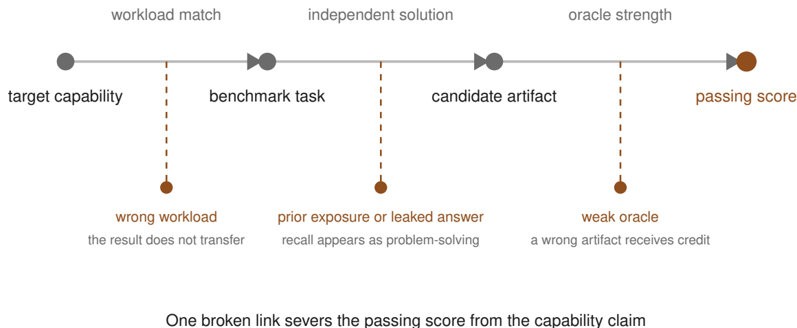
Figure 3.1: A passing score supports a capability claim only when the benchmark matches the target workload, the solution is independent of prior or in-task exposure, and the oracle rejects incorrect artifacts. A failure at any link invalidates a different inference.
