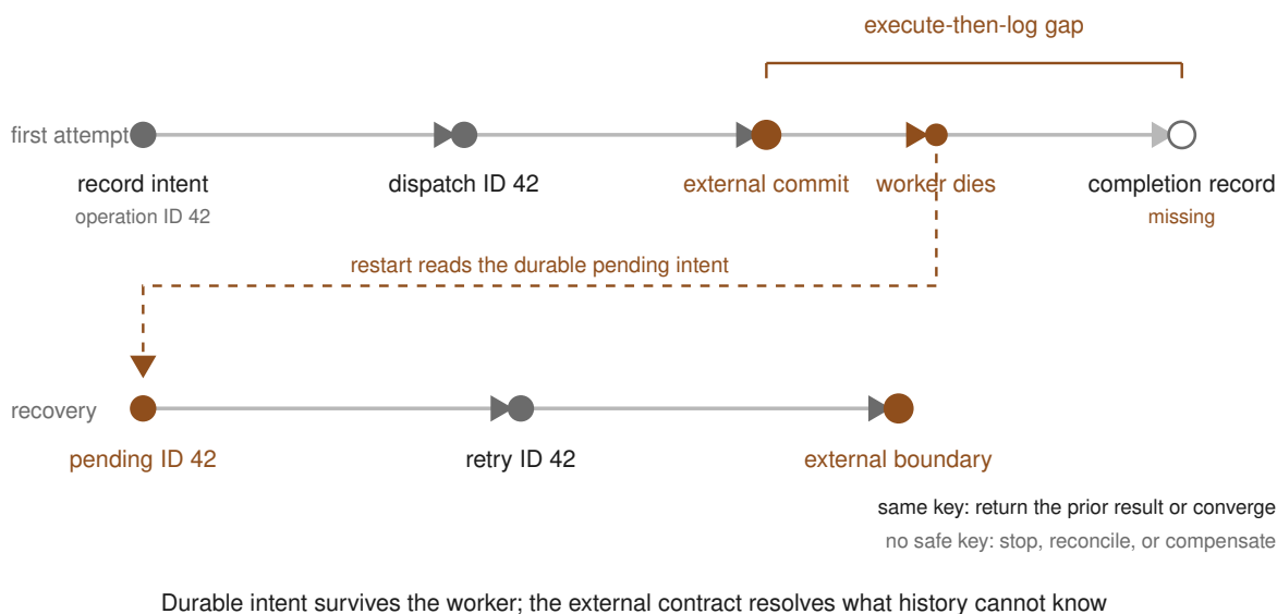
Figure 8.1: A first attempt records a durable intent and operation identity before an external commit. If the worker dies before recording completion, a replacement reads the pending intent and retries with the same identity; the external boundary must return the prior result, converge, or force explicit reconciliation.
