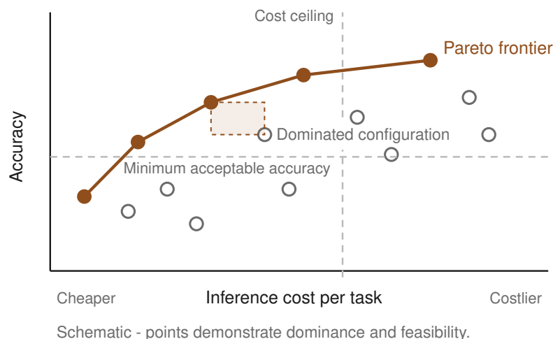
Figure 2.1: Schematic of a cost-accuracy frontier, dominated configurations, and minimum-accuracy and cost-ceiling feasibility constraints.
