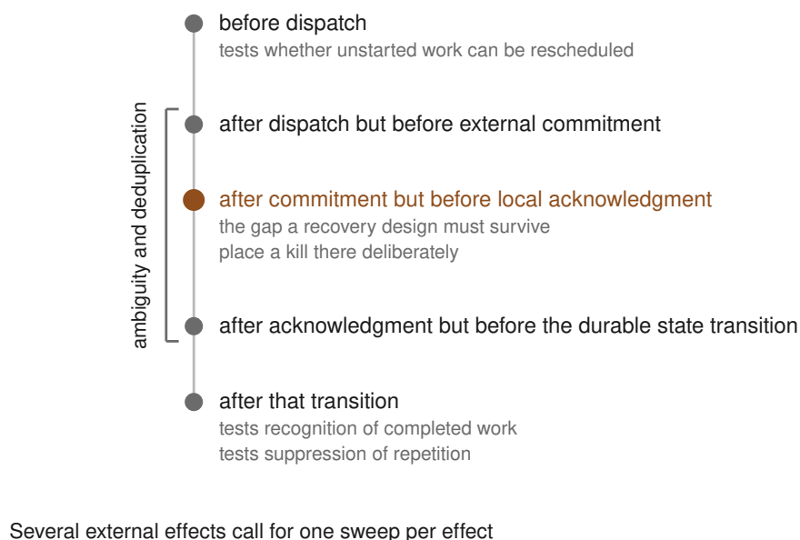
Figure 9.1: Five lifecycle kill points test recovery from unstarted work through ambiguous commitment gaps to durable completion, including recognition and suppression of repeated external effects.
