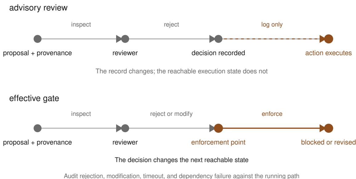
Figure 16.1: An advisory review can record rejection while leaving execution reachable. An effective gate connects the review decision to an enforcement point, so rejection or modification changes the next reachable state.
