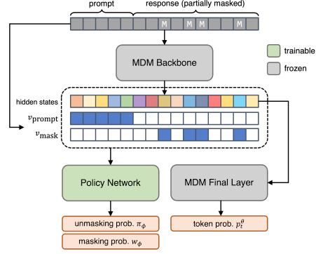
Figure 3: An illustration of the shared-torso architecture of VLP with a trained MDM.
